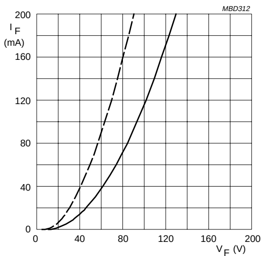
BY8016. Dotted line: T_j = 120^\circ\text{C} . Solid line: T_j = 25^\circ\text{C} .
