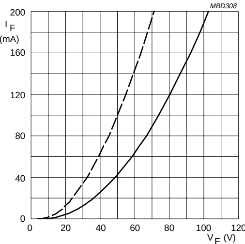
BY8012. Dotted line: T_j = 120^\circ\text{C} . Solid line: T_j = 25^\circ\text{C} .
