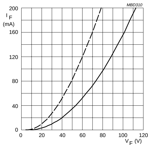
BY8014. Dotted line: T_j = 120^\circ\text{C} . Solid line: T_j = 25^\circ\text{C} .
