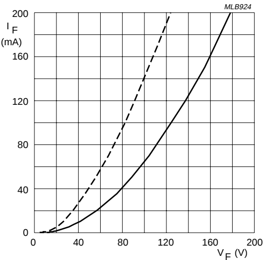
BY8114. Dotted line: T_j = 120^\circ\text{C} . Solid line: T_j = 25^\circ\text{C} .
