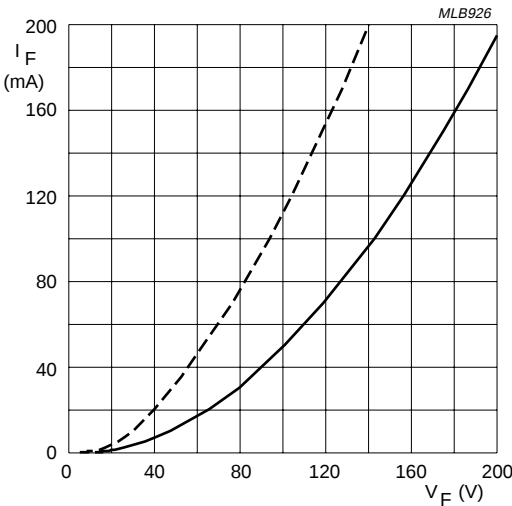
BY8116. Dotted line: T_j = 120^\circ\text{C} . Solid line: T_j = 25^\circ\text{C} .
