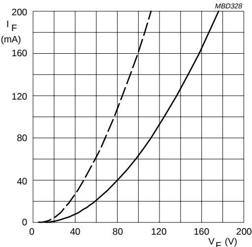
BY8418. Dotted line: T_j = 120\text{ }^{\circ}\text{C} . Solid line: T_j = 25\text{ }^{\circ}\text{C} .
