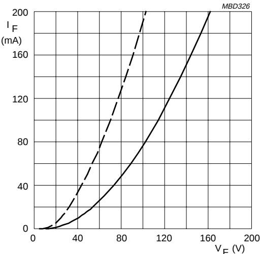
BY8416. Dotted line: T_j = 120\text{ }^{\circ}\text{C} . Solid line: T_j = 25\text{ }^{\circ}\text{C} .
