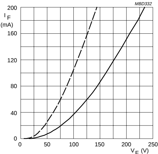
BY8424. Dotted line: T_j = 120\text{ }^{\circ}\text{C} . Solid line: T_j = 25\text{ }^{\circ}\text{C} .
