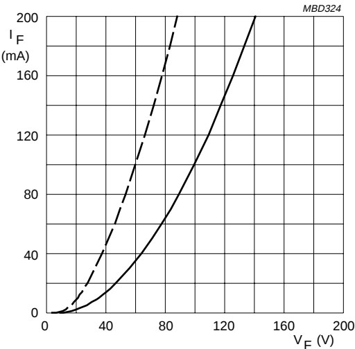
BY8414. Dotted line: T_J = 120\text{ }^{\circ}\text{C} . Solid line: T_J = 25\text{ }^{\circ}\text{C} .
