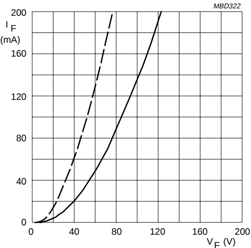
BY8412. Dotted line: T_J = 120\text{ }^{\circ}\text{C} . Solid line: T_J = 25\text{ }^{\circ}\text{C} .
