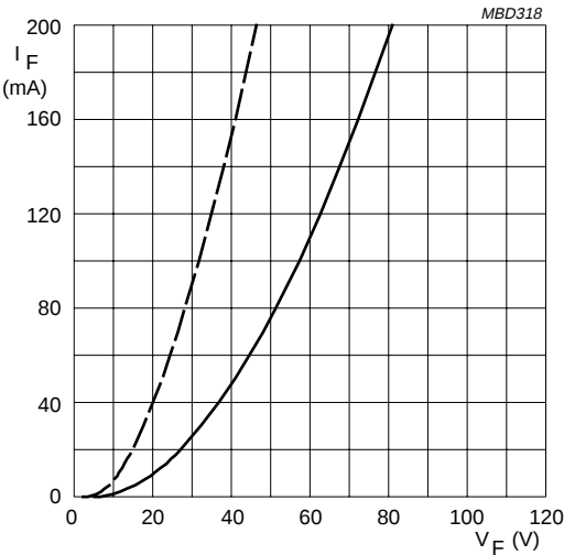
BY8408. Dotted line: T_J = 120\text{ }^{\circ}\text{C} . Solid line: T_J = 25\text{ }^{\circ}\text{C} .
