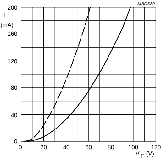
BY8410. Dotted line: T_J = 120\text{ }^{\circ}\text{C} . Solid line: T_J = 25\text{ }^{\circ}\text{C} .
