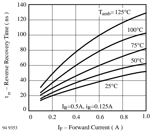
94 9353 Figure 4. Max. Reverse Recovery Time vs. Forward Current
