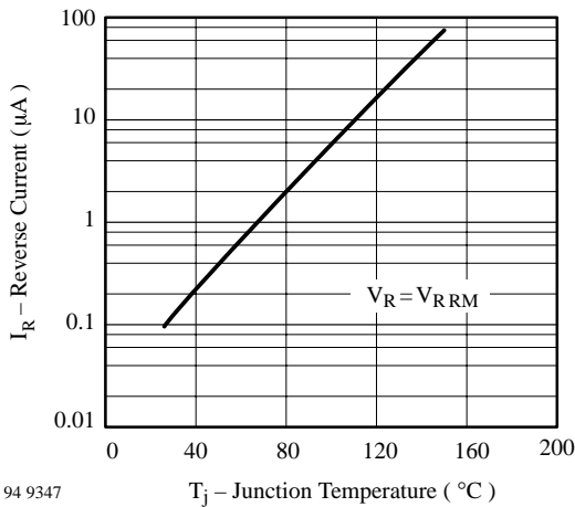
94 9347 Figure 1. Typ. Reverse Current vs. Junction Temperature
