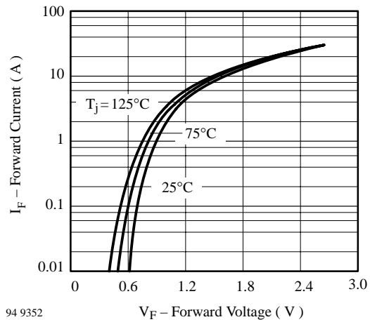
94 9352 Figure 3. Max. Forward Current vs. Forward Voltage
