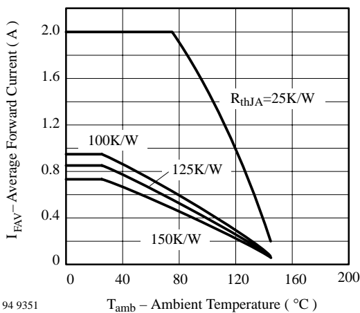
94 9351 Figure 2. Max. Average Forward Current vs. Ambient Temperature
