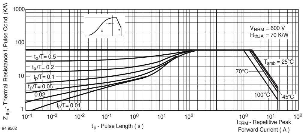
Figure 7. Thermal Response
