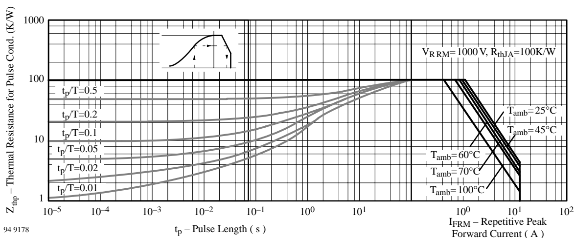
Figure 7. Thermal Response
