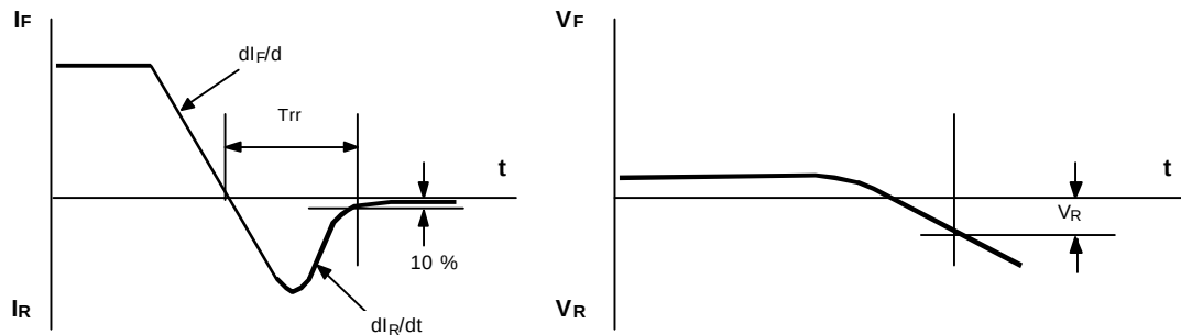
FIG.1 - REVERSE RECOVERY TIME CHARACTERISTIC
