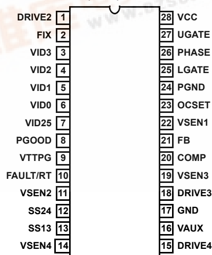
ISL6524 (SOIC) TOP VIEW
