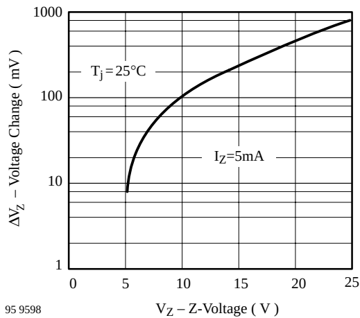
Typical Change of Working Voltage under Operating Conditions at T_{amb} = 25^\circ\text{C}
