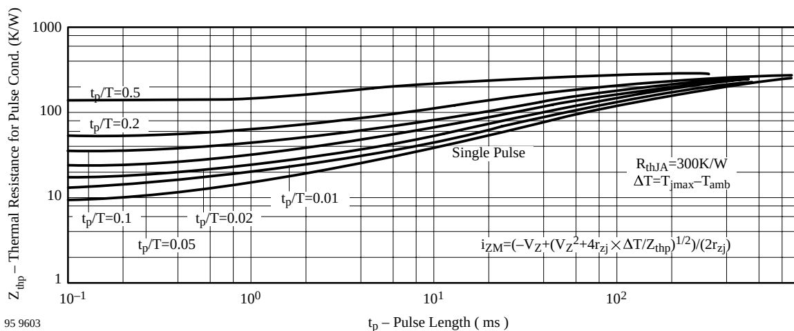
Thermal Response
