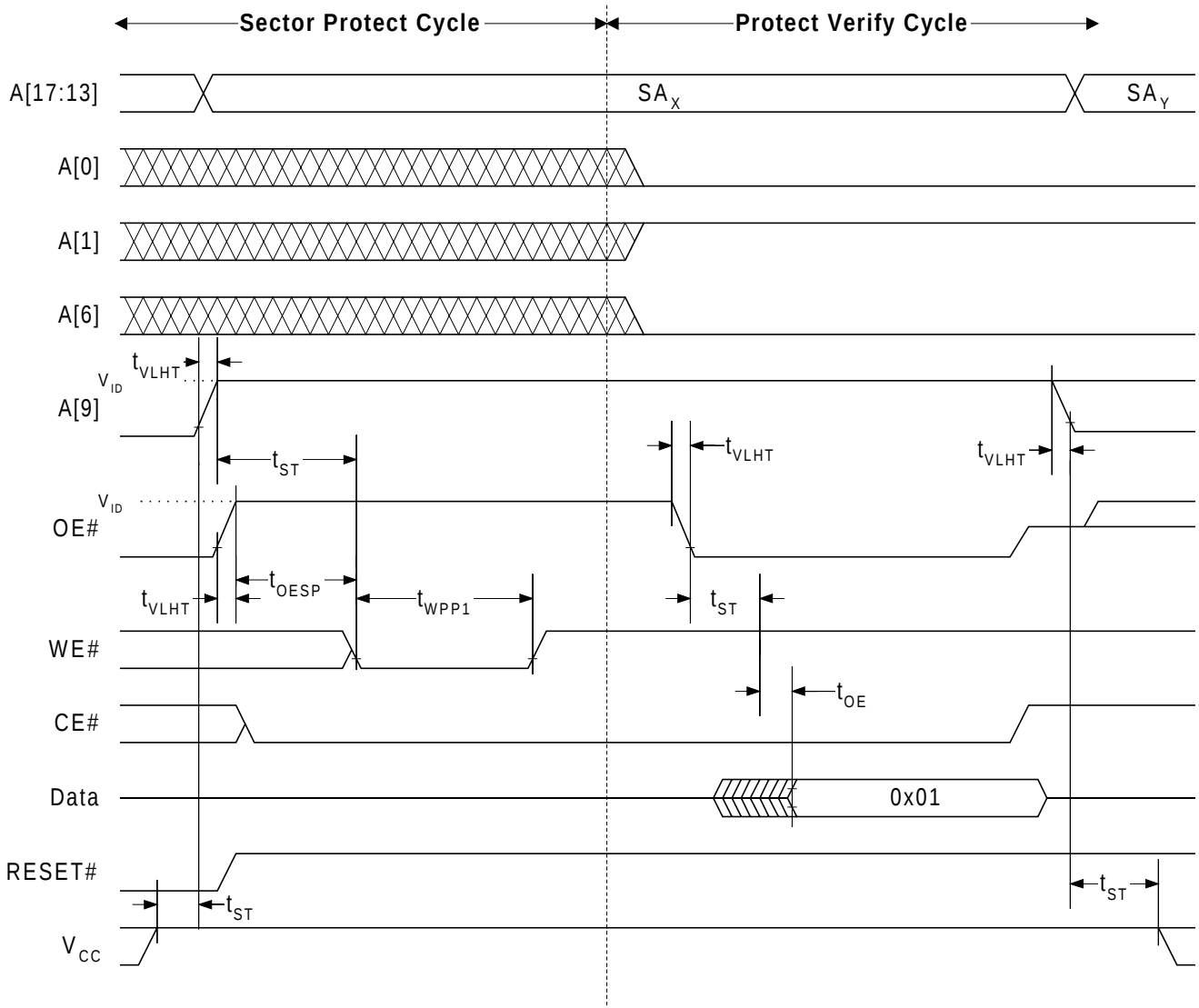
Figure 20. Sector Protect Timings
