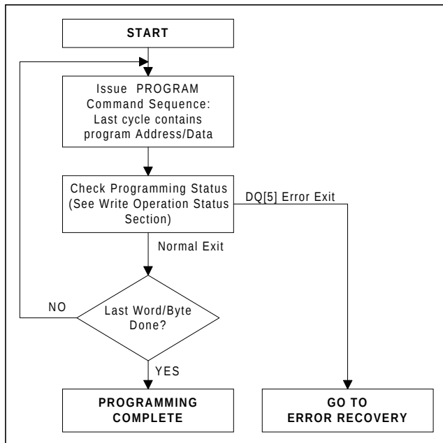
Figure 4. Programming Procedure
