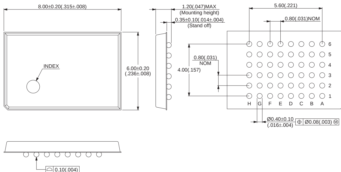
48-pin plastic FBGA (BGA-48P-M01)
