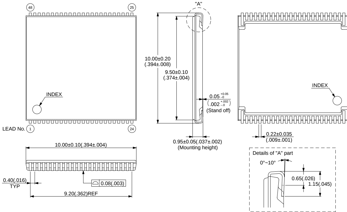
48-pin plastic CSOP (LCC-48P-M03)
