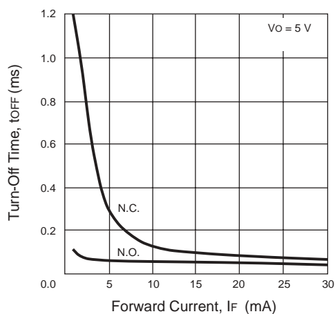
TURN-OFF TIME vs. FORWARD CURRENT
