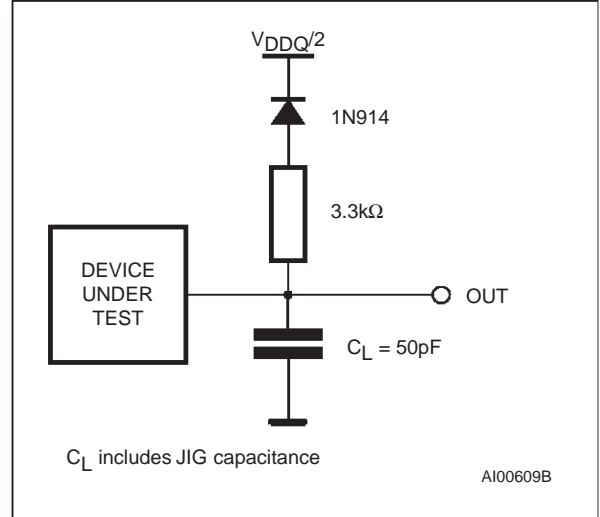
Figure 6. AC Testing Load Circuit
