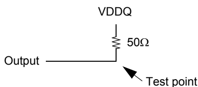
Figure 3 : Pulldown slew rate test load
