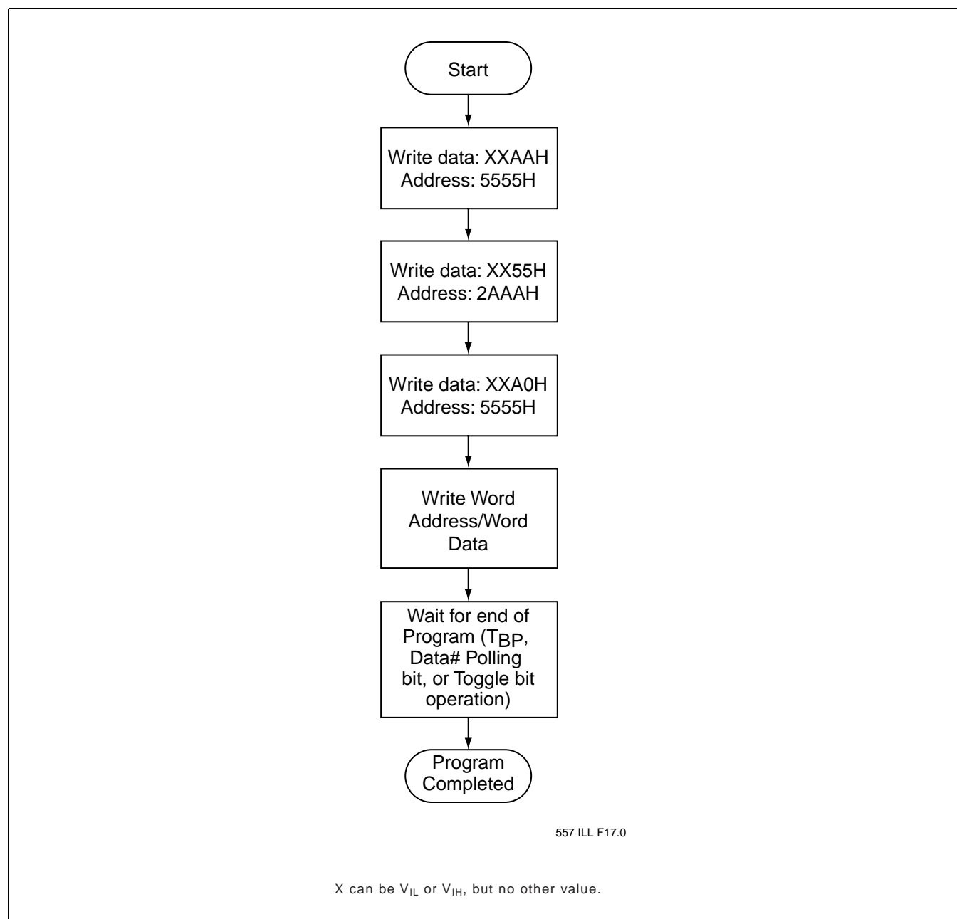
FIGURE 17: WORD-PROGRAM ALGORITHM
