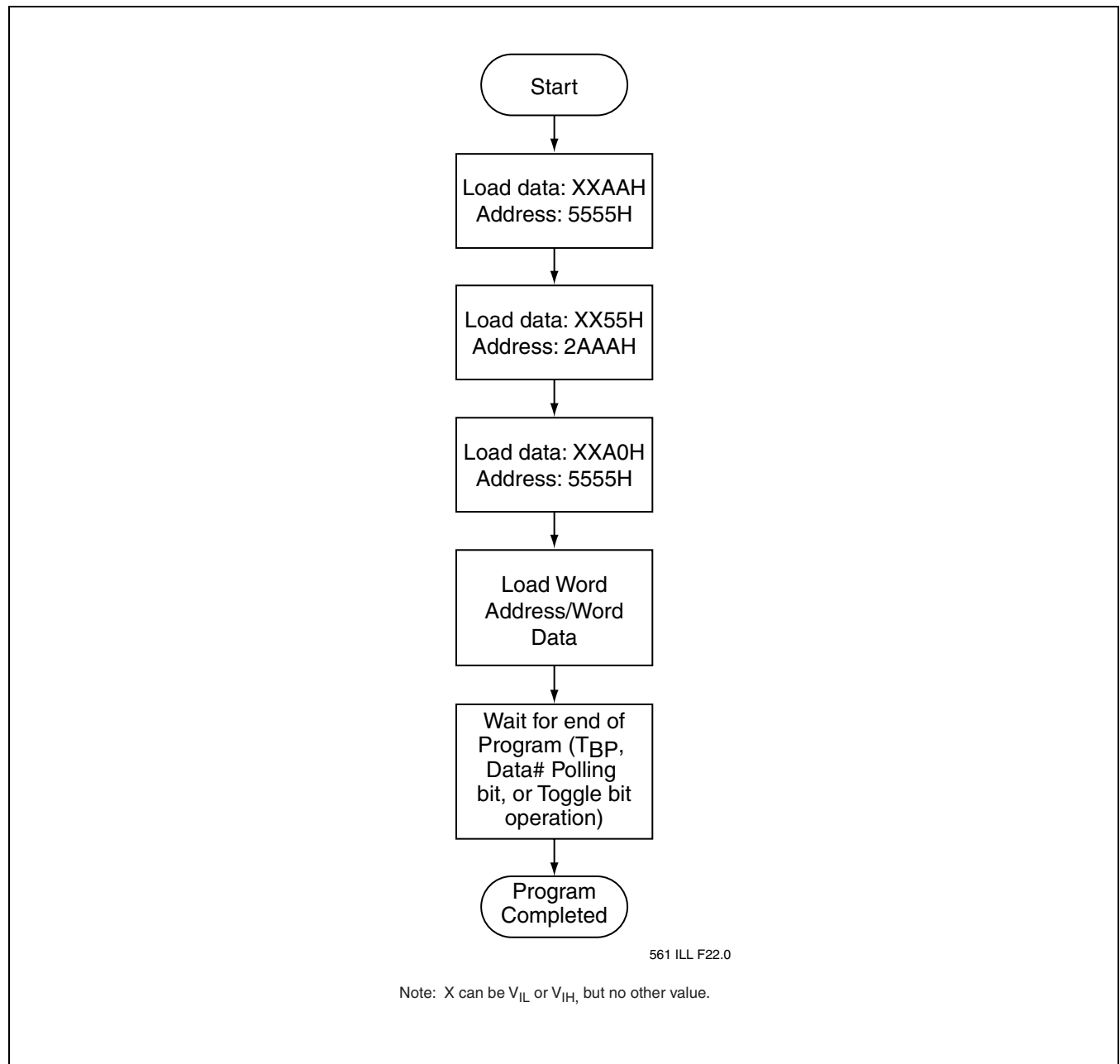
FIGURE 21: WORD-PROGRAM ALGORITHM
