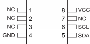
8-lead SOIC, PDIP
