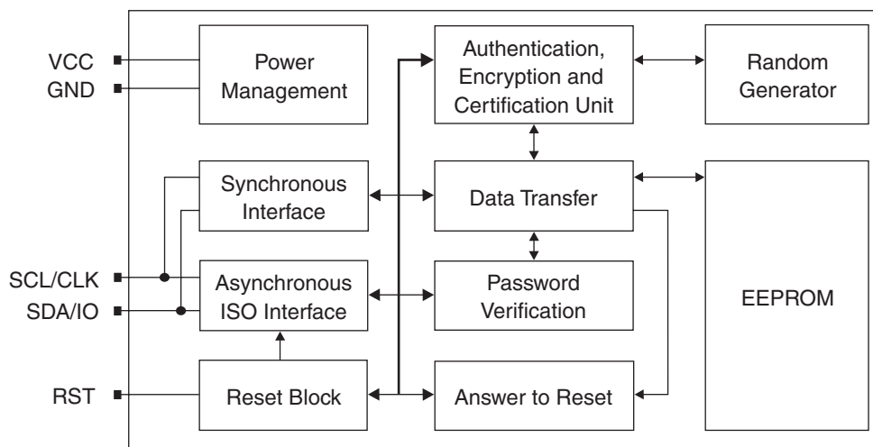
Figure 1. Block Diagram
