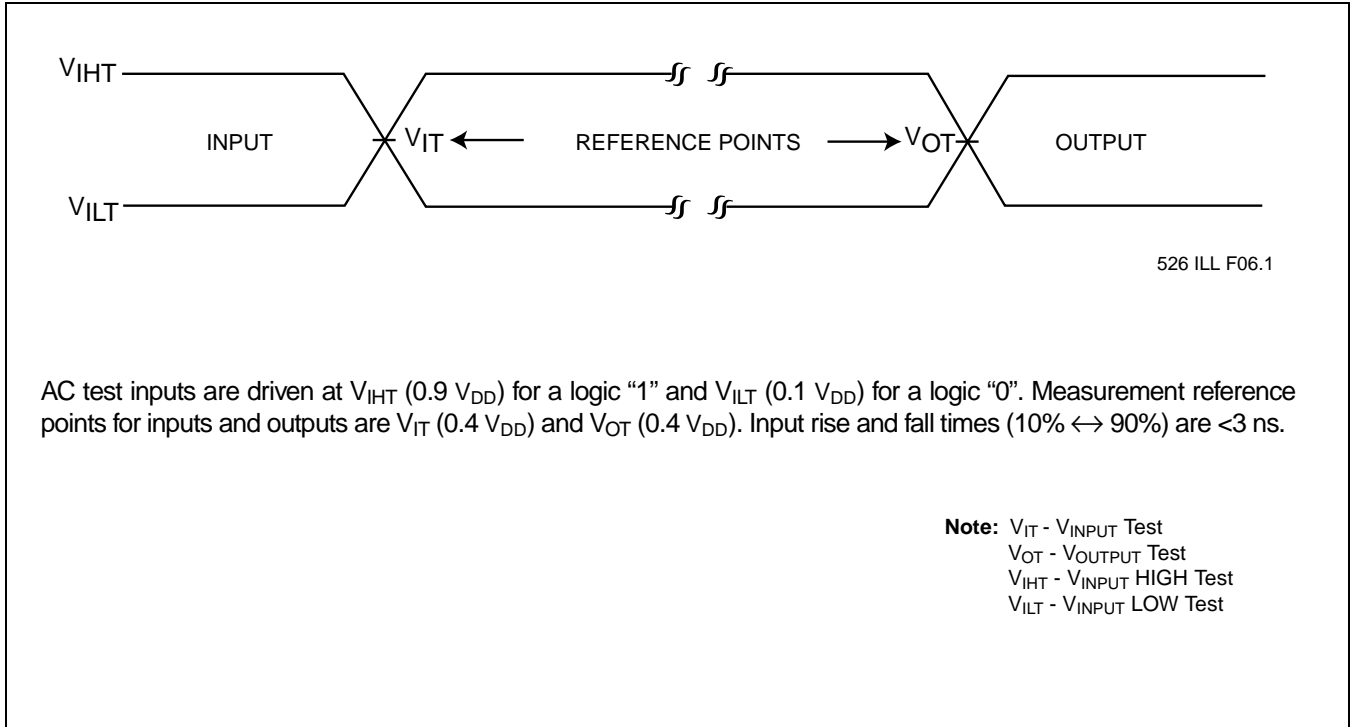
FIGURE 25: AC INPUT/OUTPUT REFERENCE WAVEFORMS (PP MODE)
