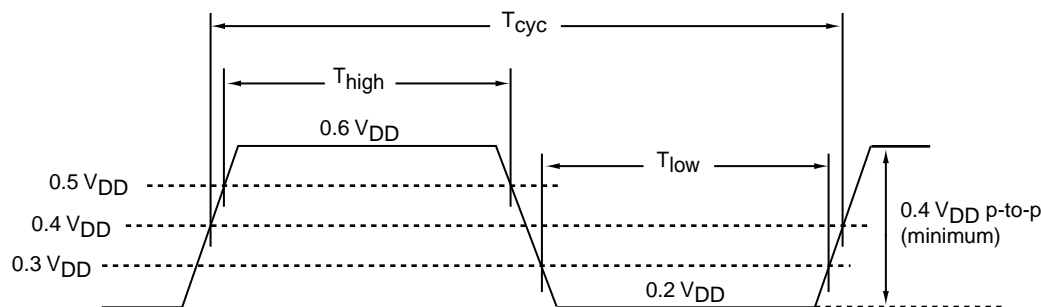
FIGURE 3: LCLK WAVEFORM
