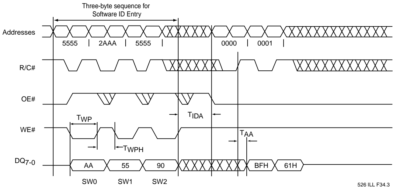
FIGURE 23: SOFTWARE ID ENTRY AND READ (PP MODE)
