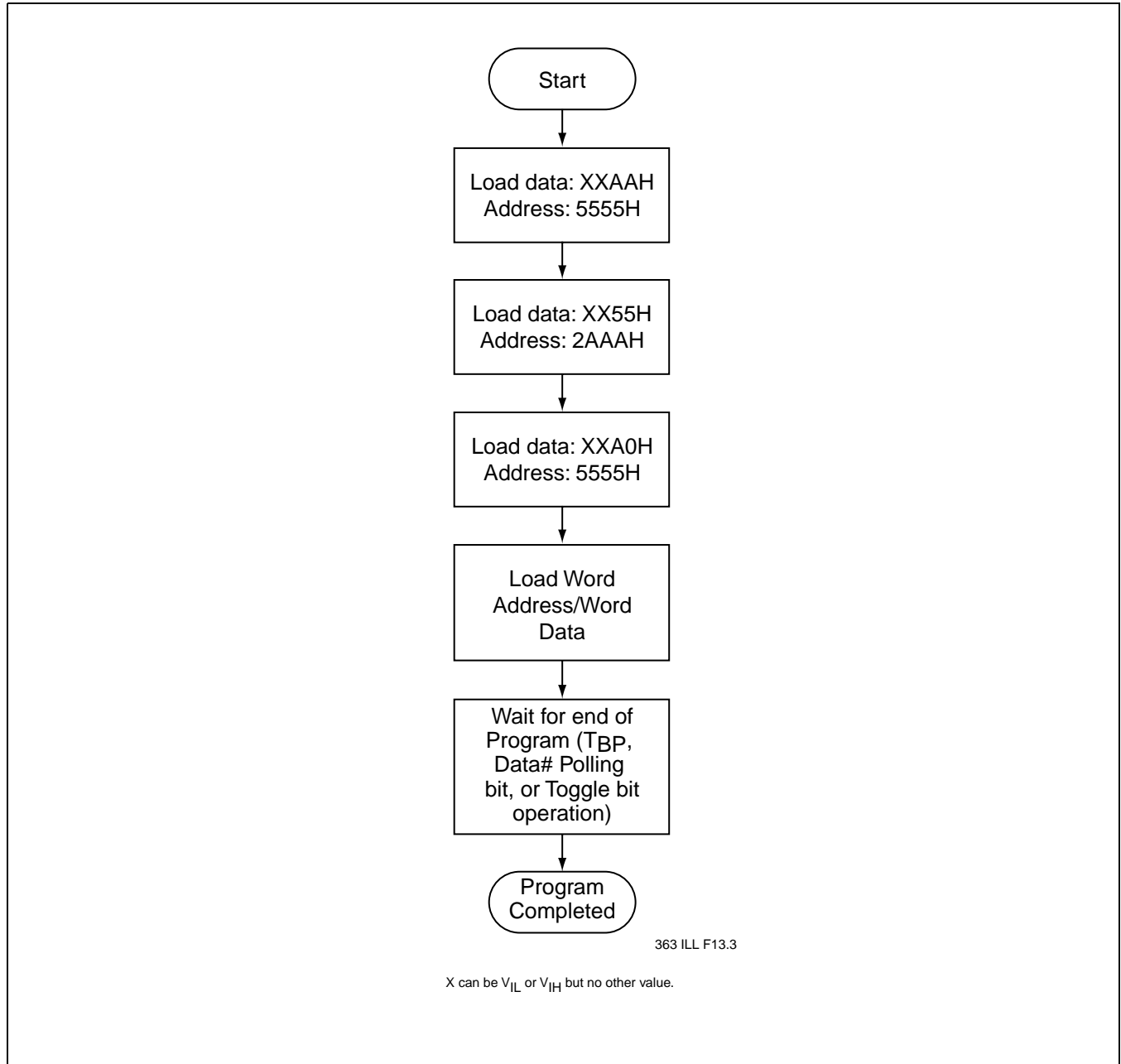
FIGURE 13: WORD-PROGRAM ALGORITHM
