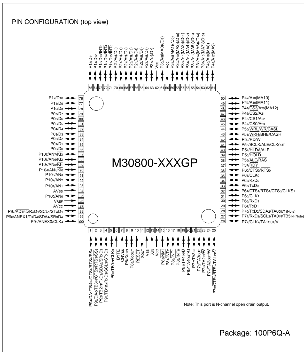
Figure 1.1.2. Pin configuration (top view)
