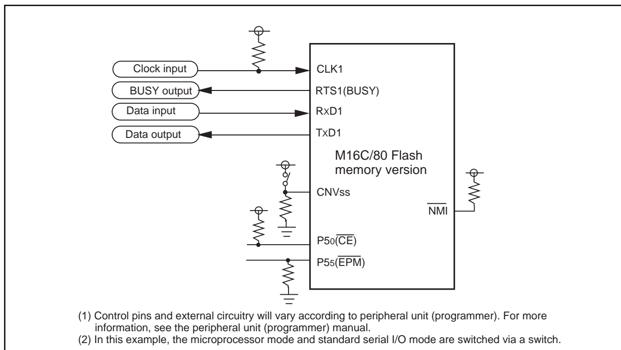
Figure 1.32.21. Example circuit application for the standard serial I/O mode 1
