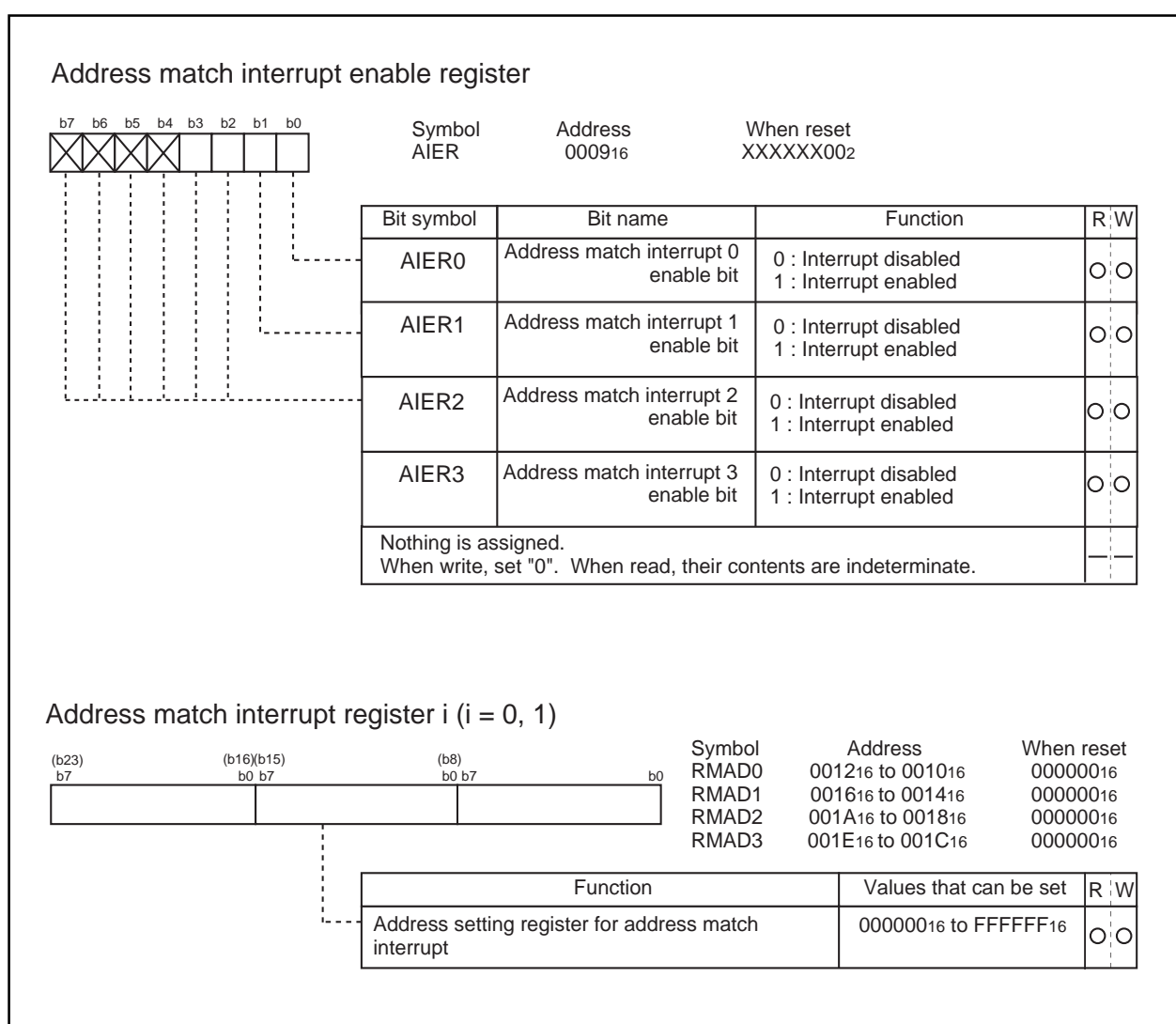
Figure 1.9.11. Address match interrupt-related registers
