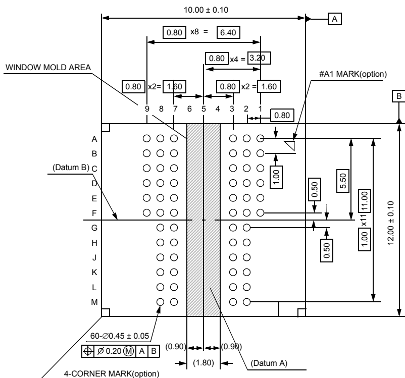
Bottom view
