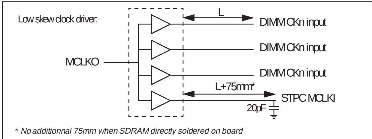
Figure 6-11. Clock routing
