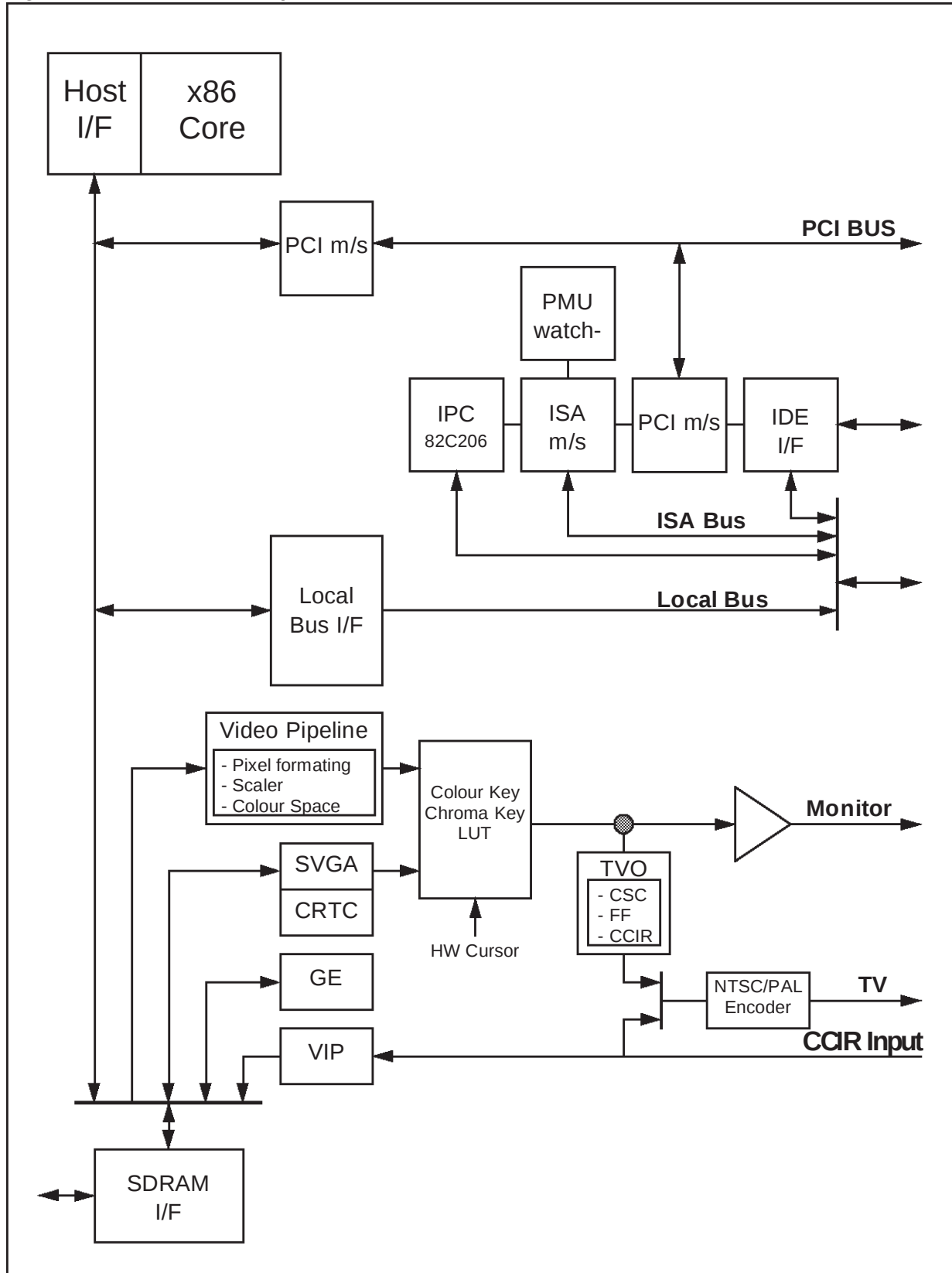
Figure 2. Functionnal description.
