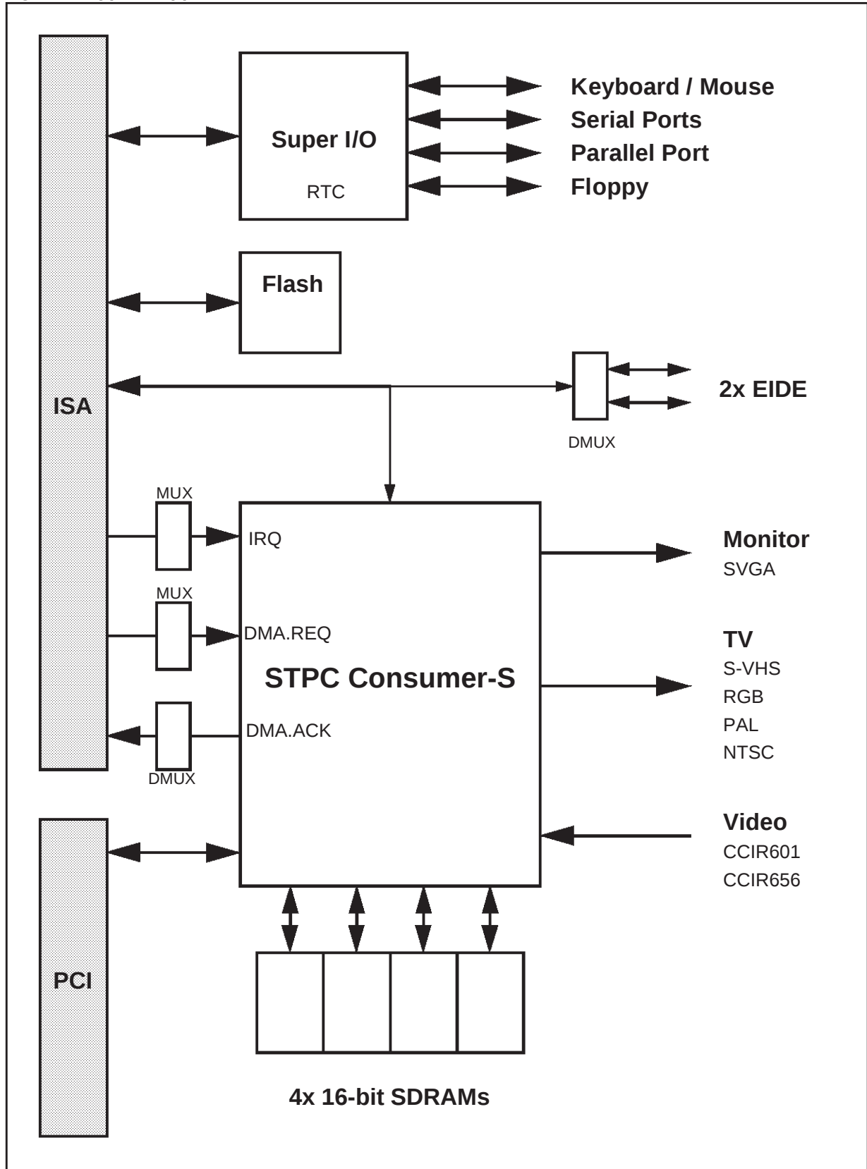
Figure 3. Typical Application
