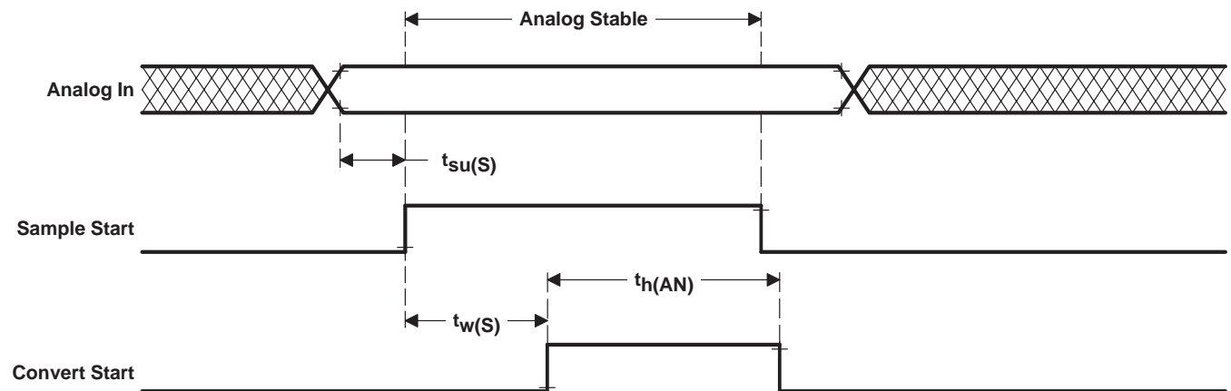
Figure 22. Analog Timing
