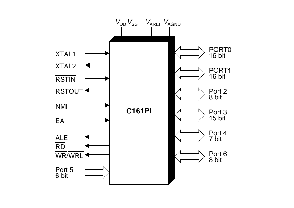
Figure 1 Logic Symbol
