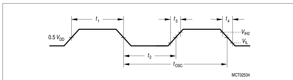
Figure 152 External Clock Drive XTAL1
