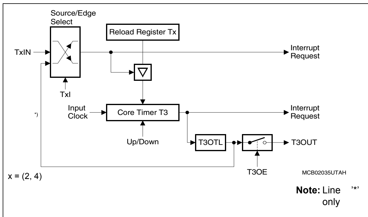
Figure 69 GPT1 Auxiliary Timer in Reload Mode
