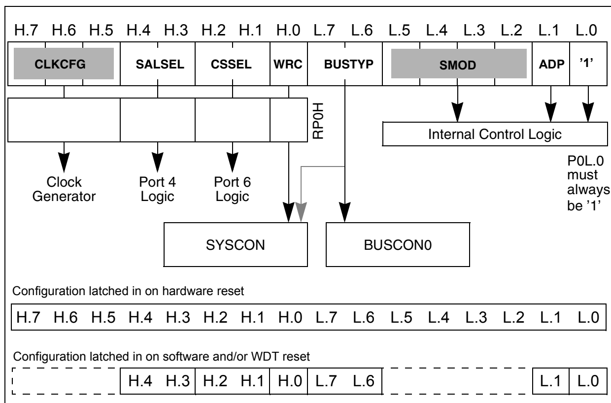
Figure 140 PORT0 Configuration during Reset
