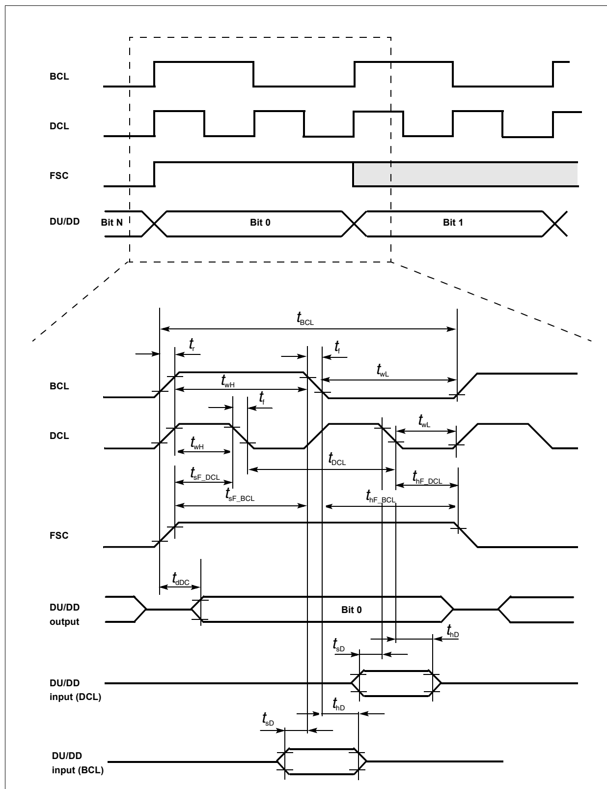
Figure 153 IOM-2 Interface Timing
