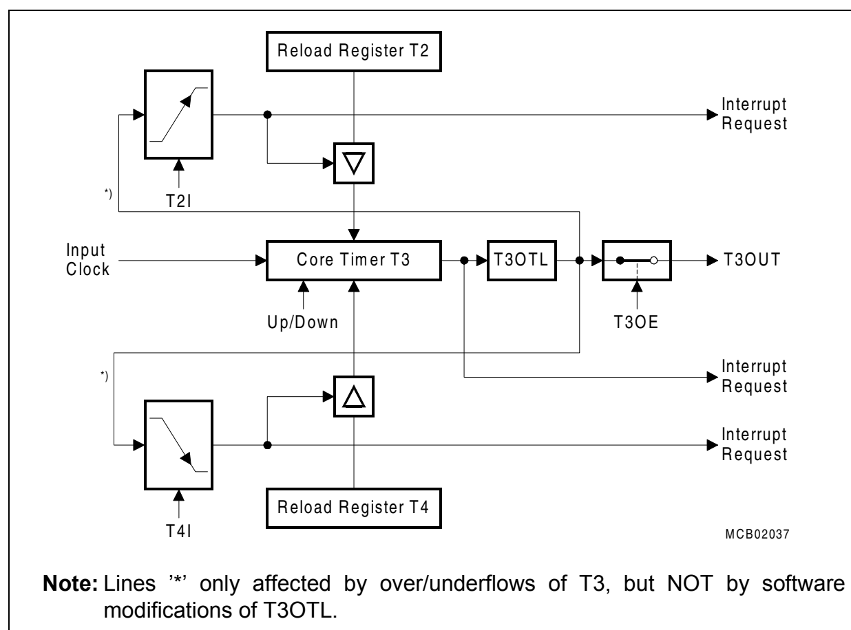
Figure 70 GPT1 Timer Reload Configuration for PWM Generation
