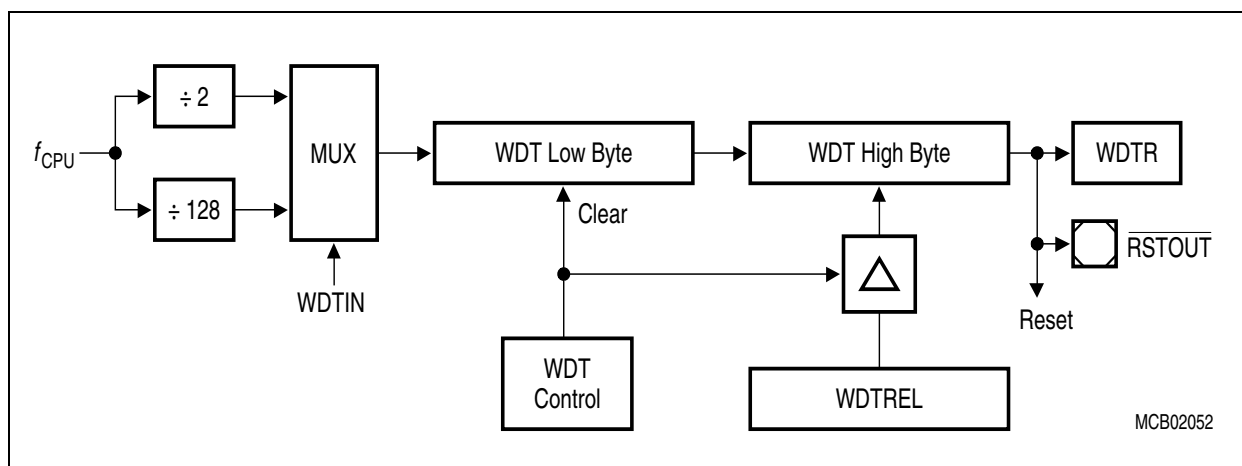
Figure 134 Watchdog Timer Block Diagram
