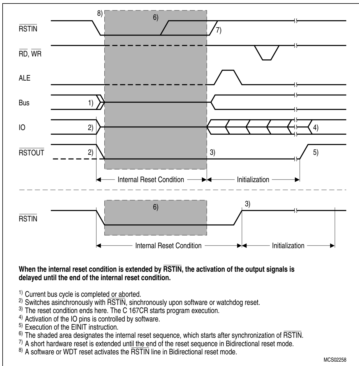
Figure 139 Reset Input and Output Signals
