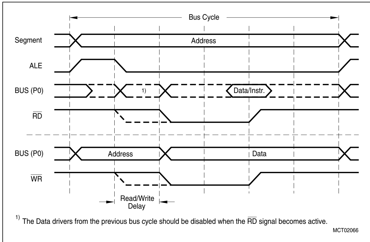
Figure 52 Read/Write Delay
