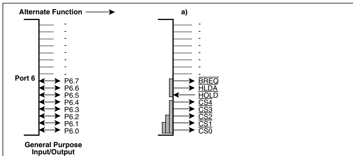
Figure 40 Port 6 I/O and Alternate Functions
