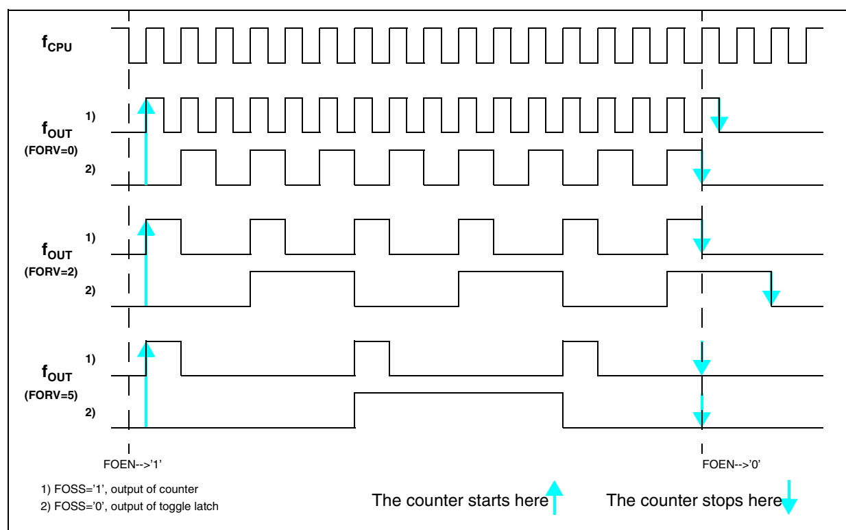
Figure 144 Signal Waveforms
