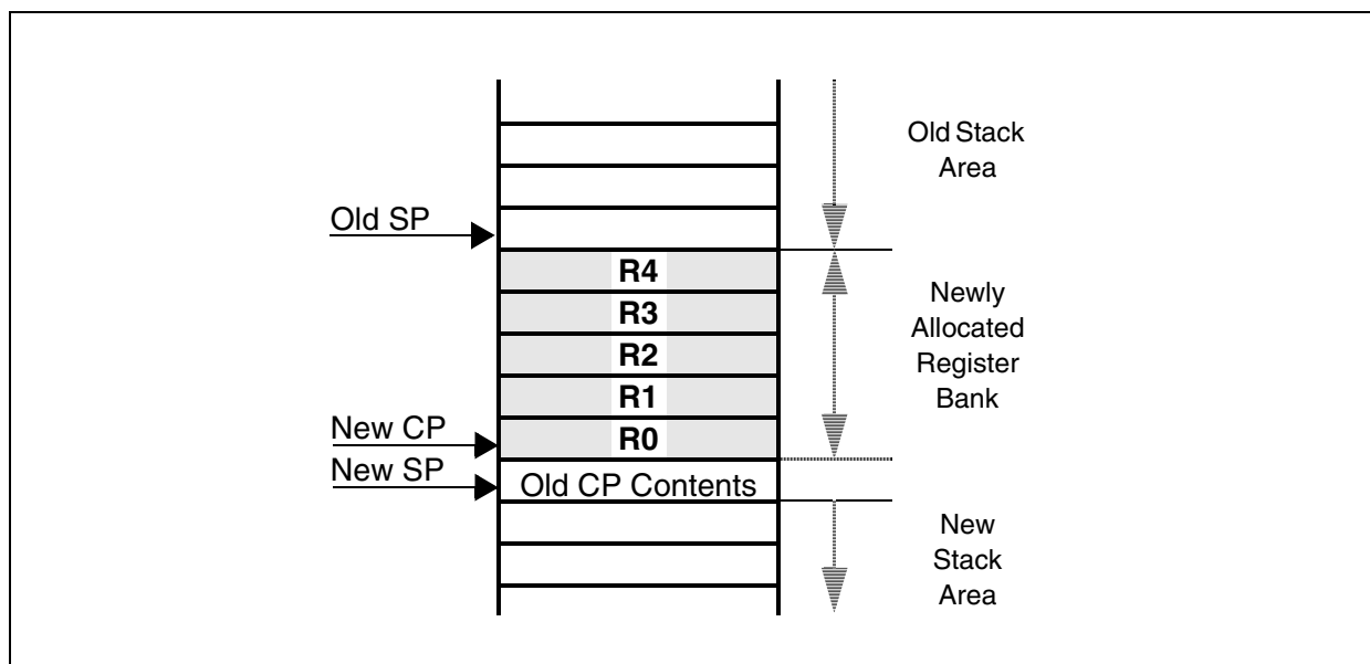
Figure 147 Local Registers
