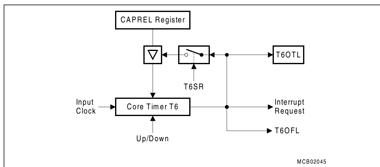
Figure 76 Timer Block 2 Register CAPREL in Reload Mode
