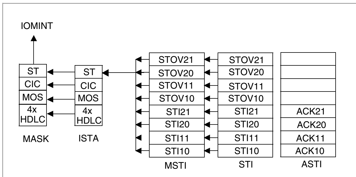
Figure 124 Interrupt Structure of the Synchronous Data Transfer
