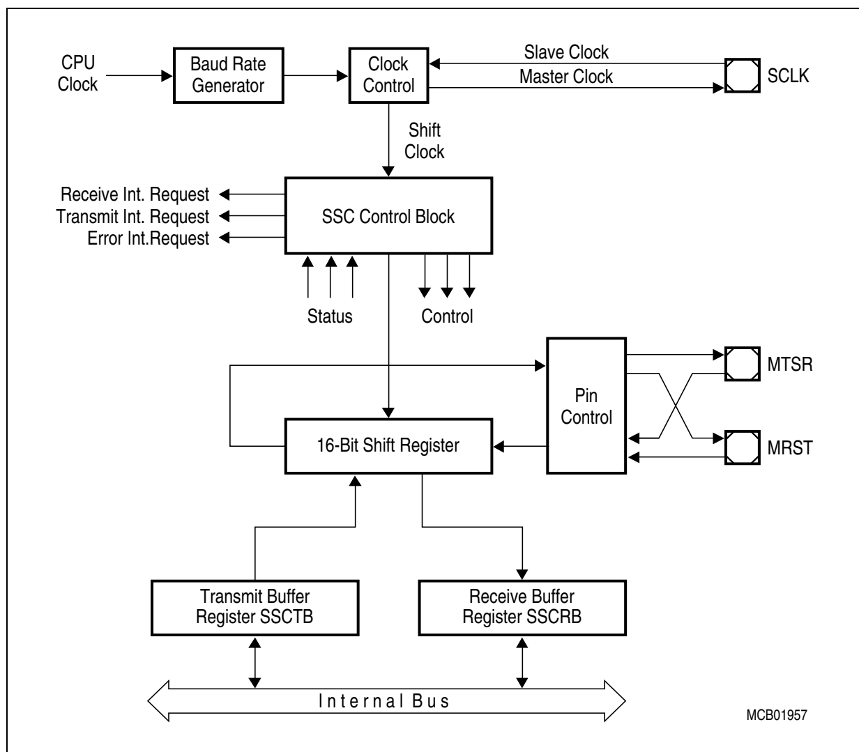
Figure 98 Synchronous Serial Channel SSC Block Diagram
