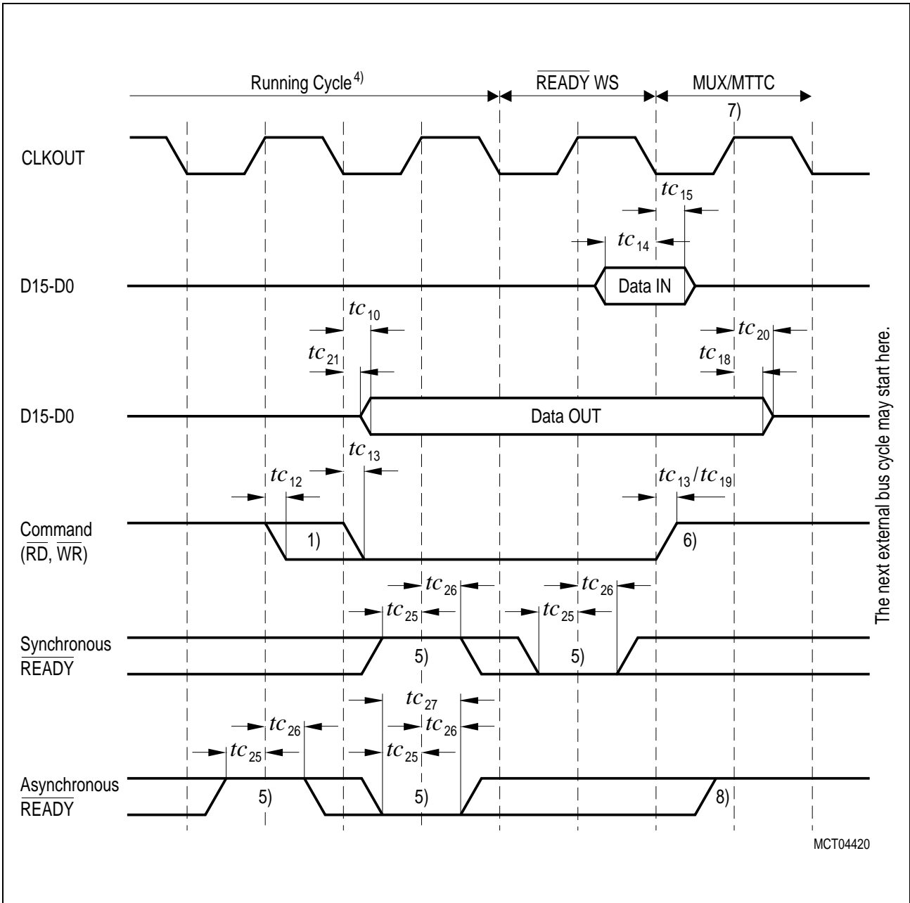
Figure 21 READY Timing
