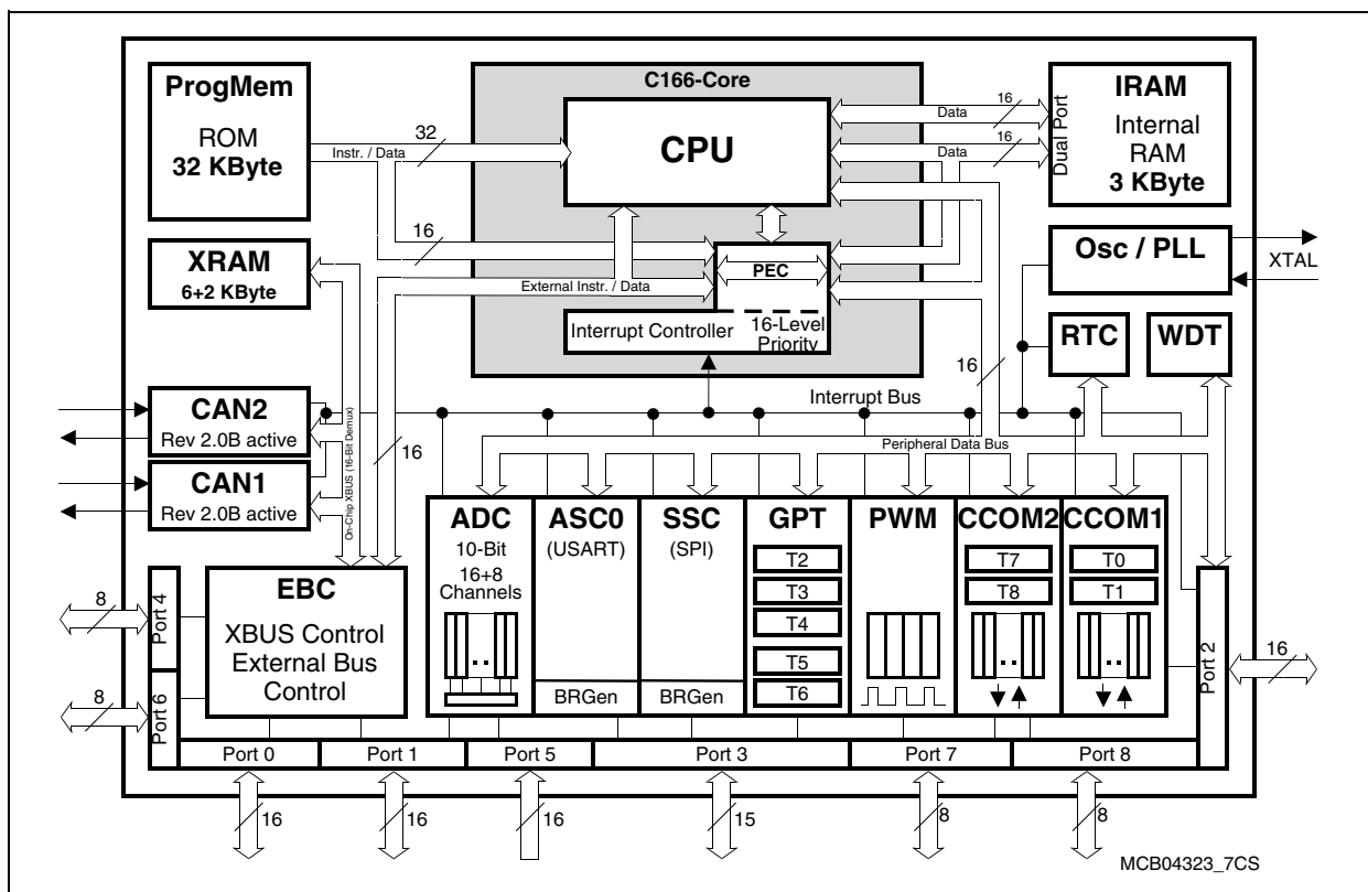
Figure 3 Block Diagram
