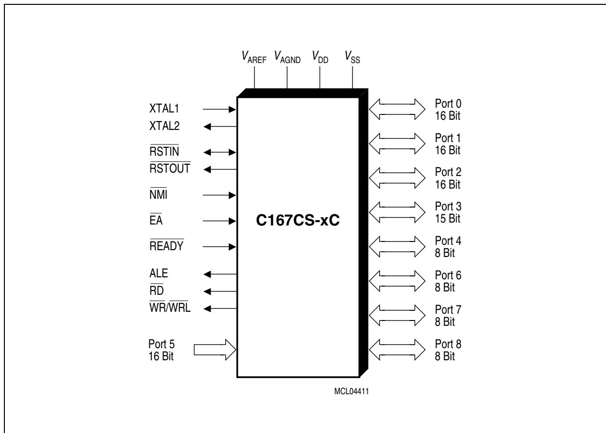
Figure 1 Logic Symbol
