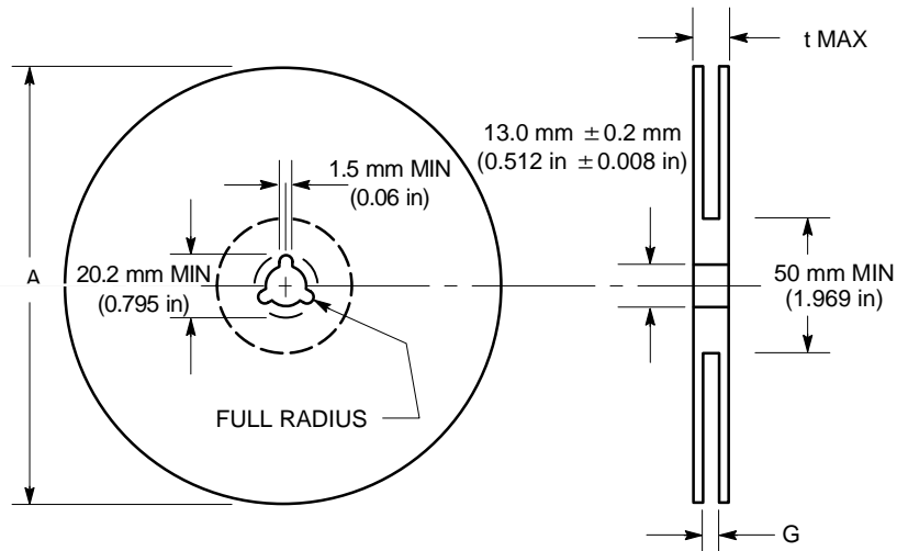
Figure 9. Reel Dimensions
