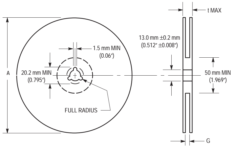
Figure 5. Reel Dimensions
