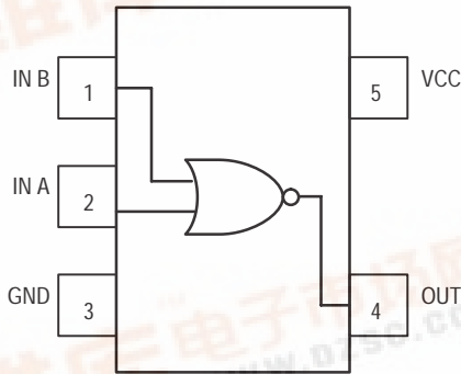
Figure 1. 5-Lead SOT-353 Pinout (Top View)
