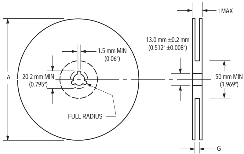
Figure 6. Reel Dimensions
