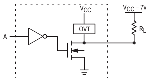
Figure 2. Output Voltage Mismatch Application
