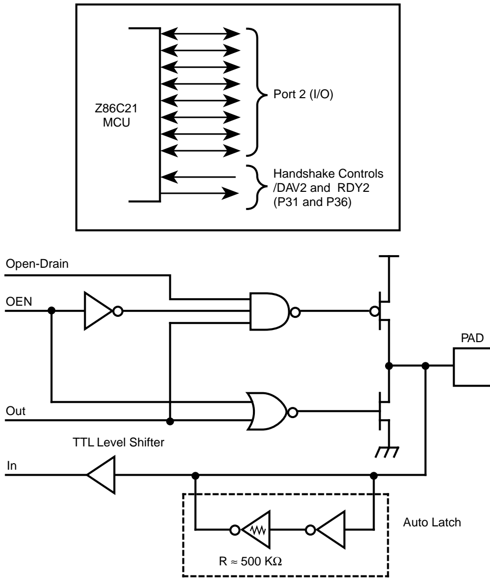
Figure 7. Port 2 Configuration
