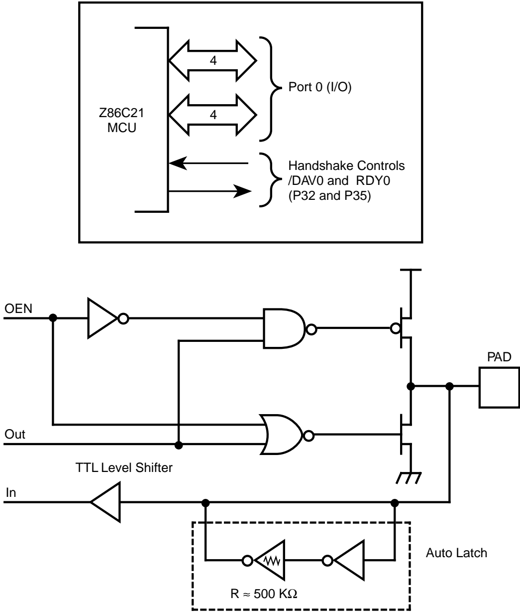
Figure 5. Port 0 Configuration
