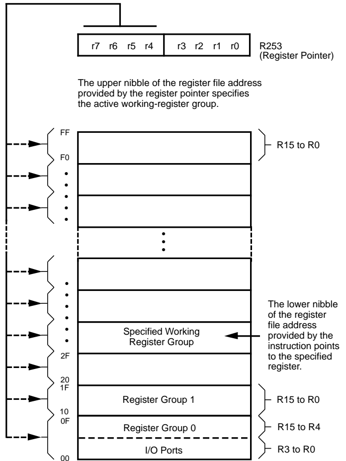
Figure 13. Register Pointer
