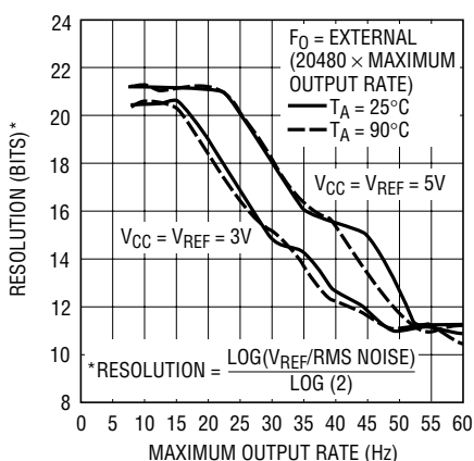
Figure 6. Resolution vs Maximum Output Rate
