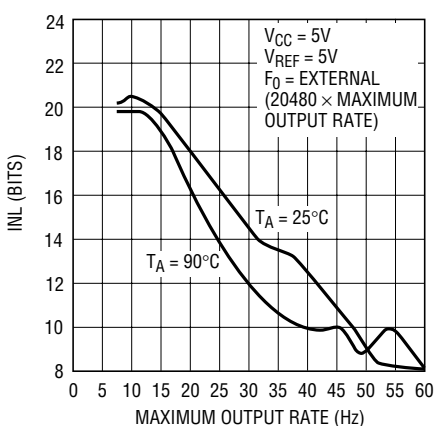
Figure 5. INL vs Maximum Output Rate
