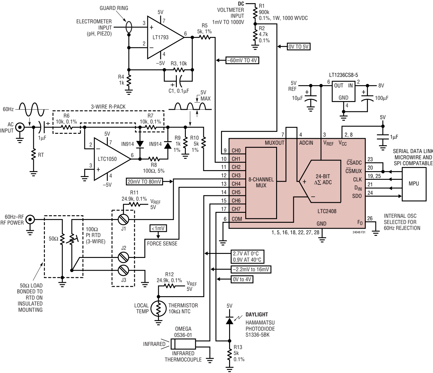
Figure 31. Measure DC to Daylight Using the LTC2408
