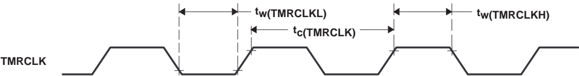
Figure 35. External Timer Clock Input Timings
