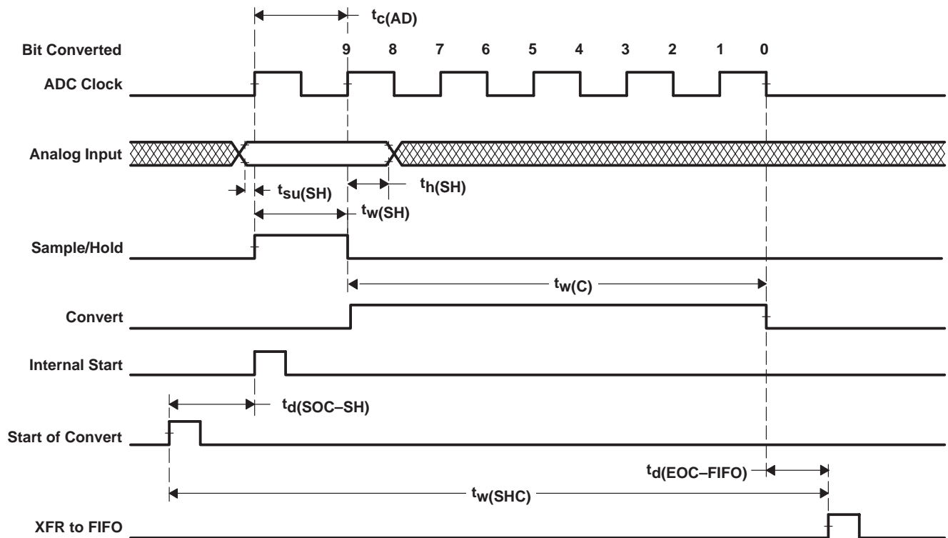
Figure 48. Analog-to-Digital Timing
