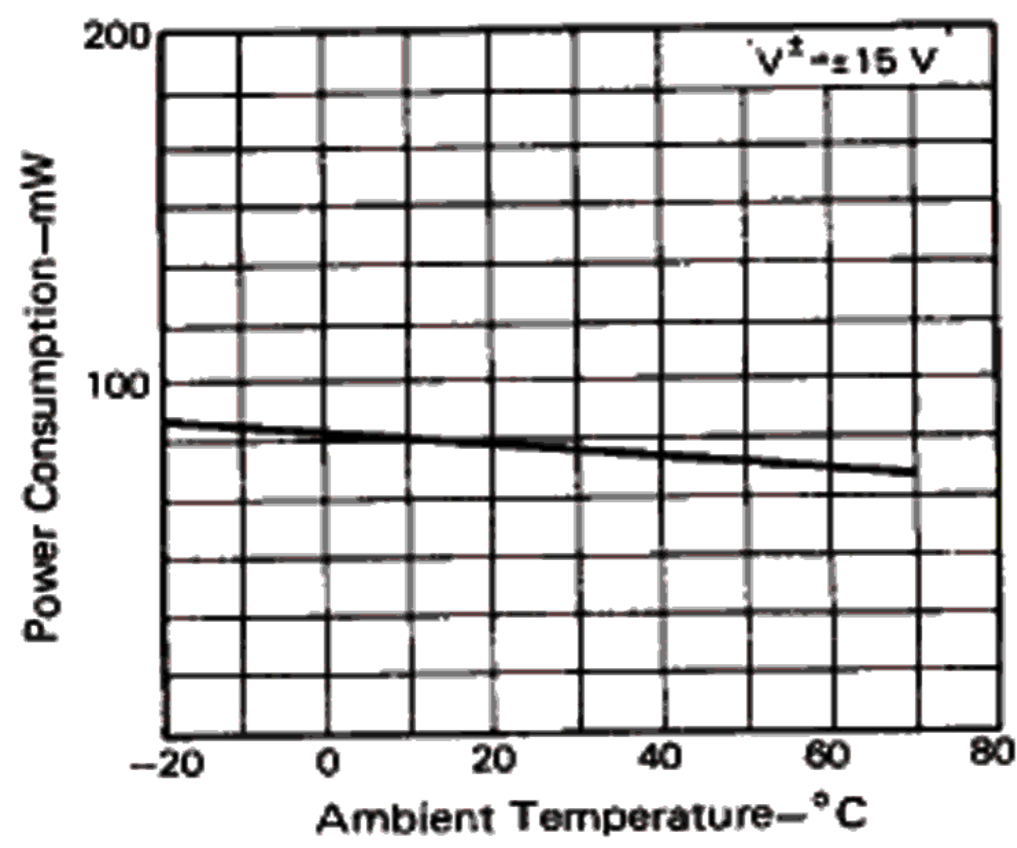
POWER CONSUMPTION
