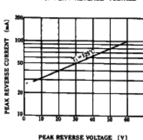
FIG.3-PEAK REVERSE CURRENT VS. PEAK REVERSE VOLTAGE
