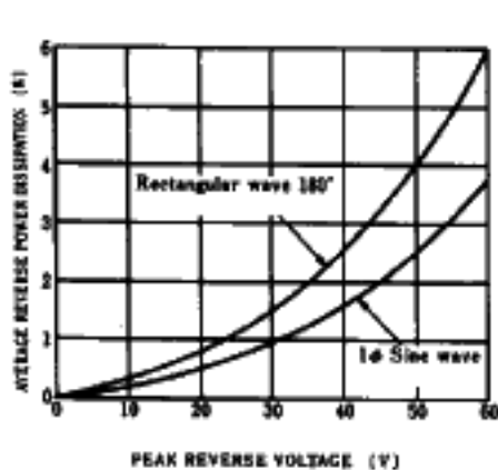
FIG.4-AVERAGE REVERSE POWER DISSIPATION
