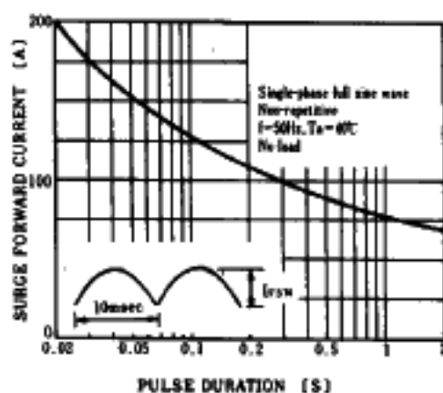
FIG.6-SURGE CURRENT RATINGS
