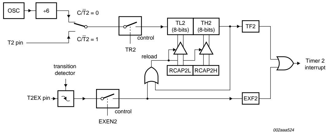
Fig 13. Timer 2 in auto-reload mode (DCEN = 0)
