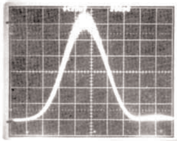
Figure 7. Avalanche Photodiode Response to a 100 ps Laser Pulse as Measured with a 350 ps Sampling Head. (Horizontal Axis: 200 ps/Division)
