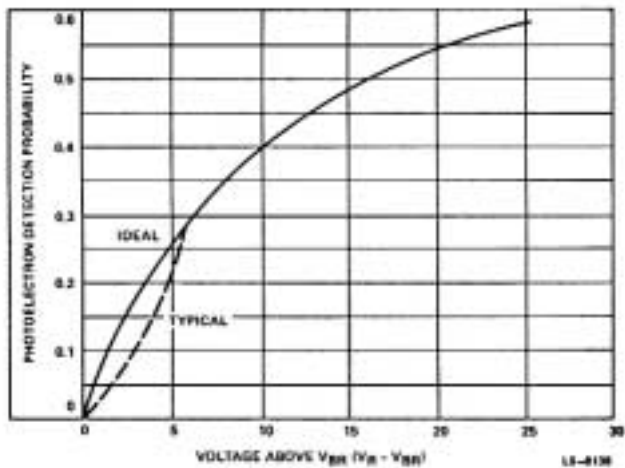
Figure 8. Geiger Mode, Photoelectron Detection Probability vs. Voltage Above V_{BR} ( V_R > V_{BR} )
