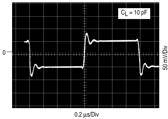
Figure 26. Small Signal
