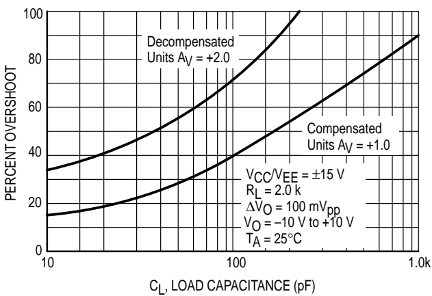
Figure 18. Percent Overshoot versus Load Capacitance
