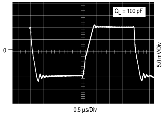
Figure 27. Large Signal
