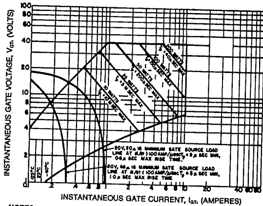
GATE CHARACTERISTICS
