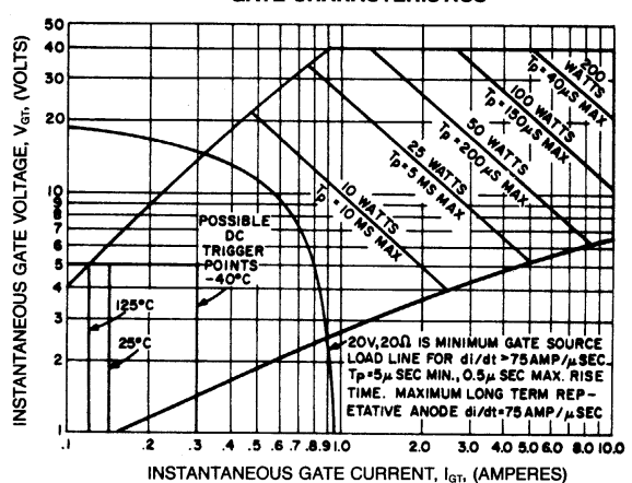
GATE CHARACTERISTICS
