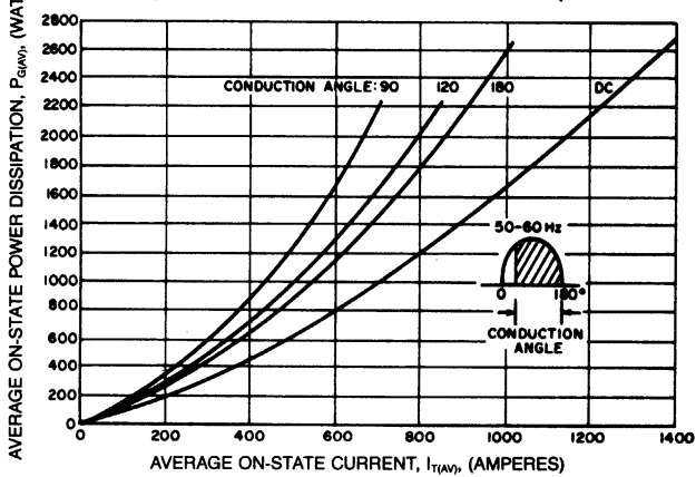
MAXIMUM ON-STATE POWER DISSIPATION (SINUSOIDAL WAVEFORM — EXTENDED)
