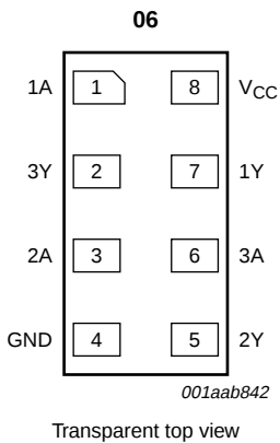
Fig 5. Pin configuration XSON8.
