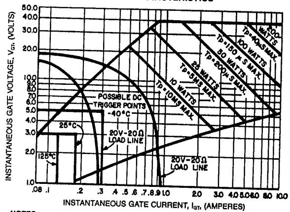
GATE CHARACTERISTICS
