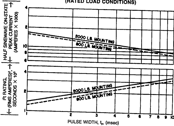
SUB-CYCLE SURGE AND I TR RATINGS (RATED LOAD CONDITIONS)
