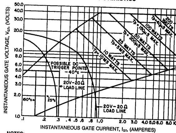
GATE CHARACTERISTICS
