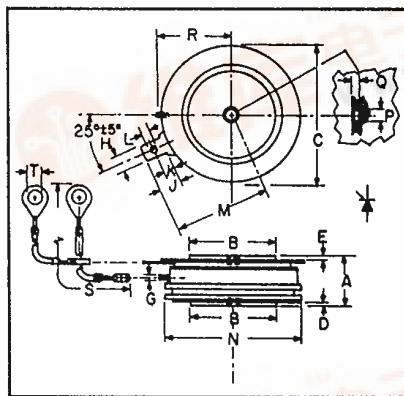
C430__X555 Outline Drawing
