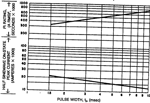
SUB-CYCLE SURGE AND I RT RATINGS (RATED LOAD CONDITIONS)
