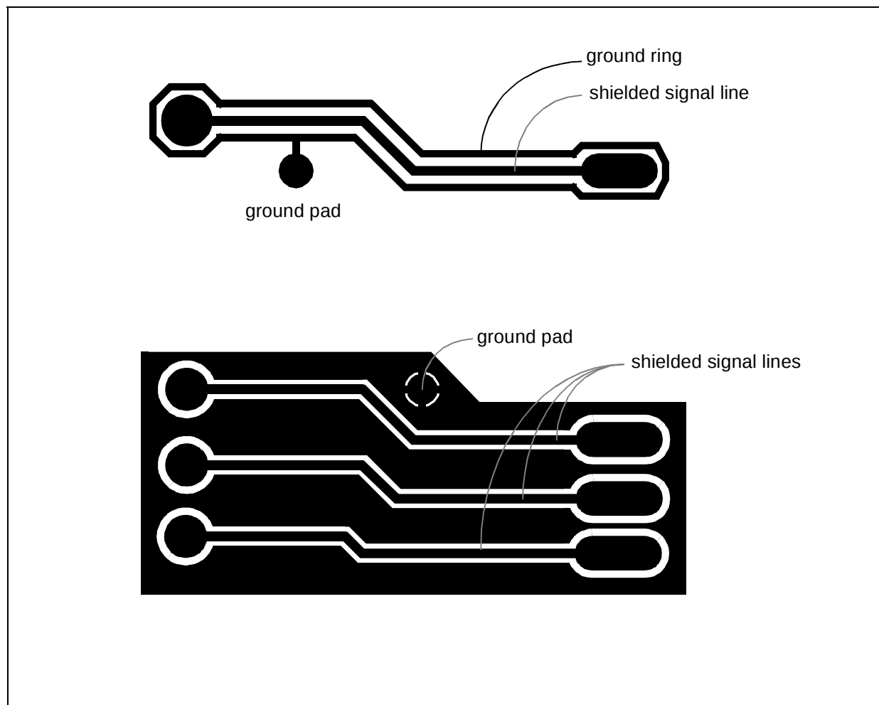
Figure 6-17. Shielding signals
