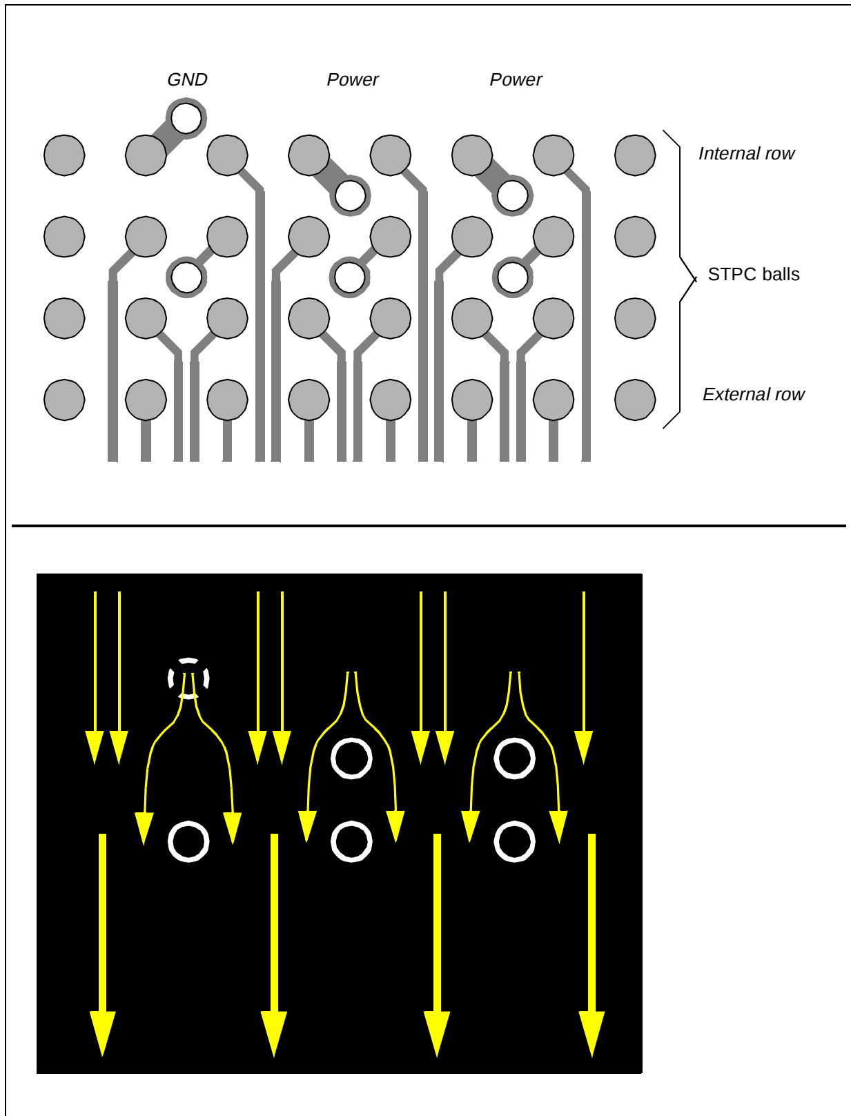
Figure 6-32. Recommend signal wiring (top &amp; ground layers) with corresponding heat flow
