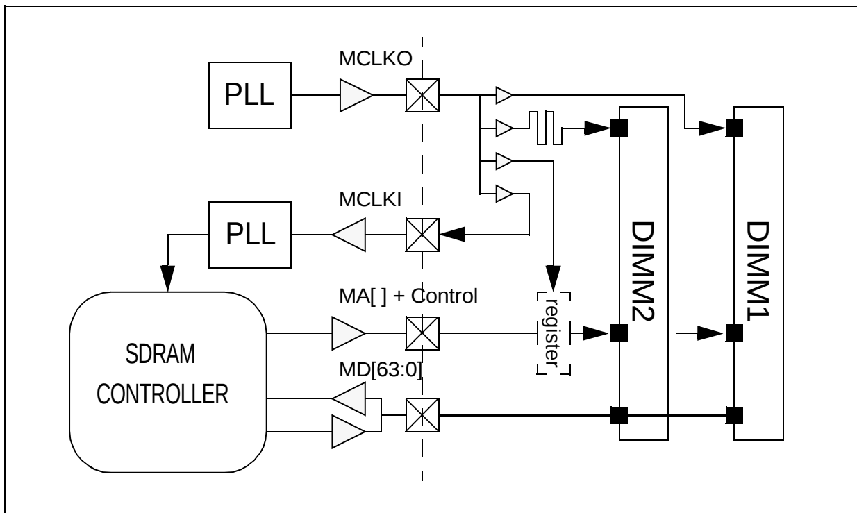
Figure 6-18. Clock Scheme
