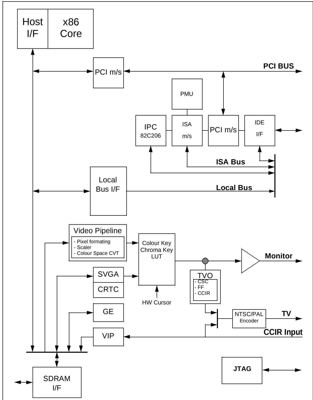
Figure 1-1. Functional description.
