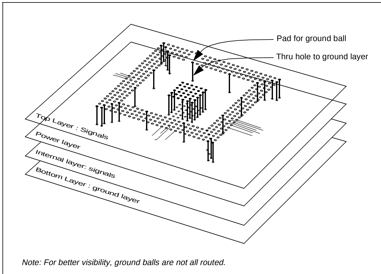
Figure 6-26. Ground routing
