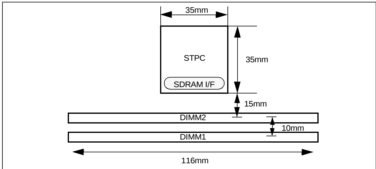
Figure 6-19. DIMM placement
