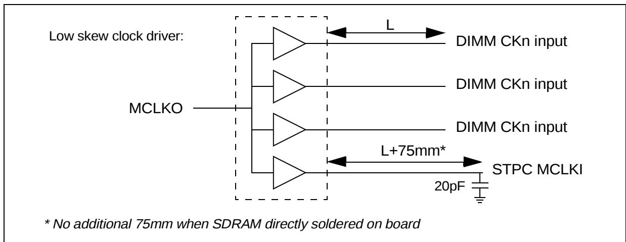
Figure 6-20. Clock Routing
