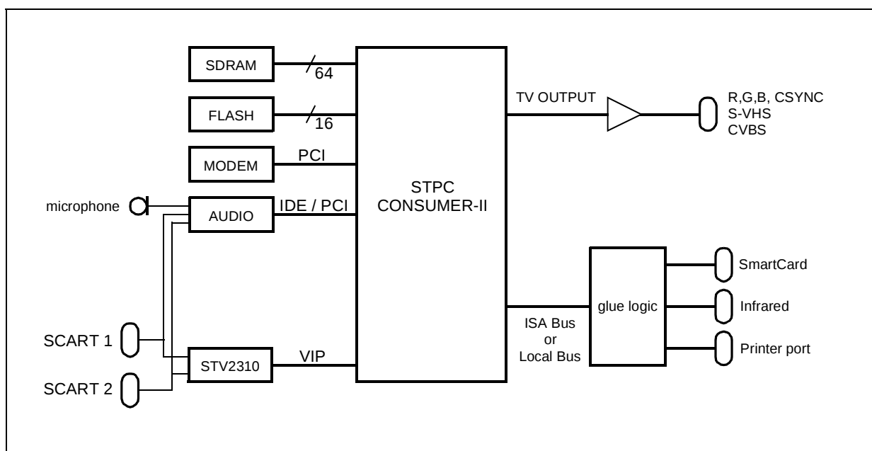
Figure 6-1. Web Box
