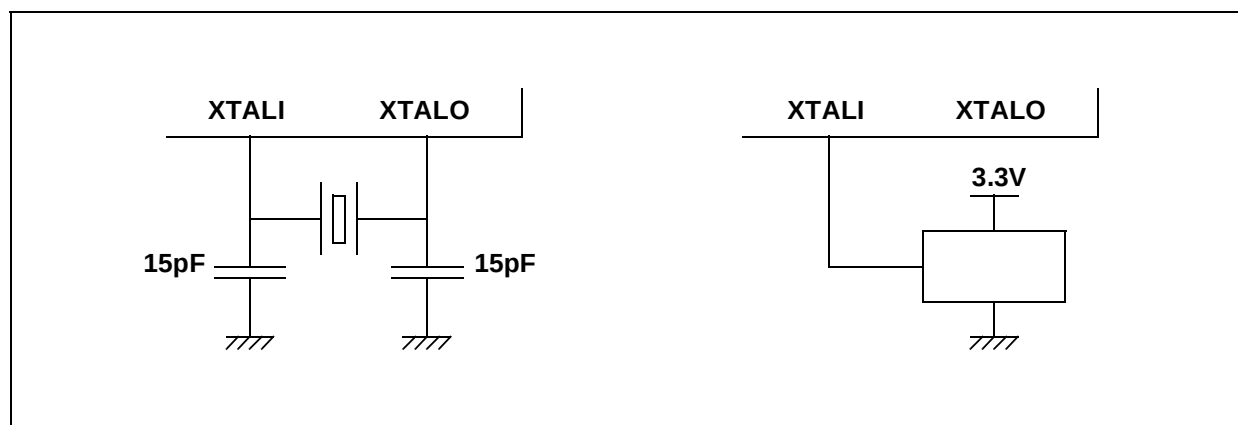
Figure 6-3. 14.31818 MHz stage
