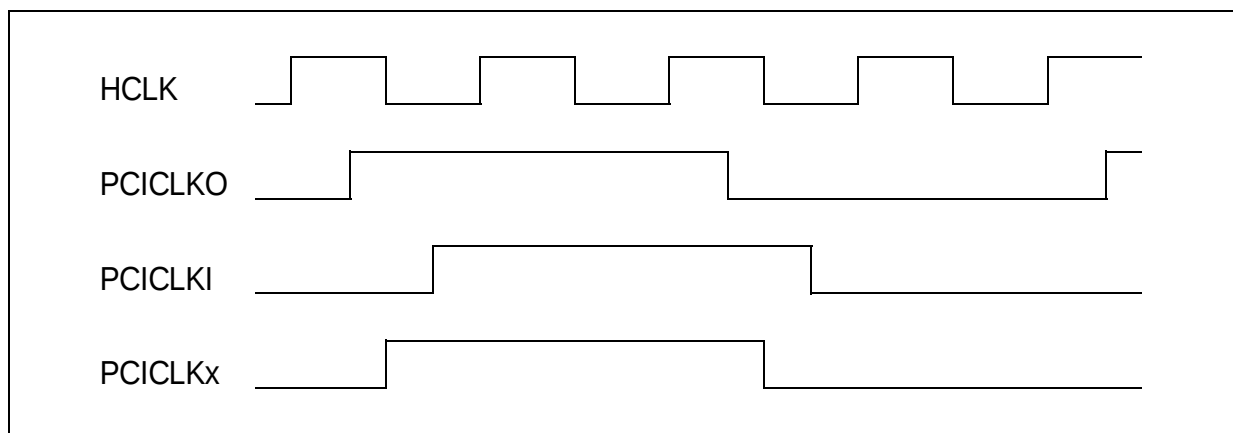
Figure 6-25. Clocks relationships
