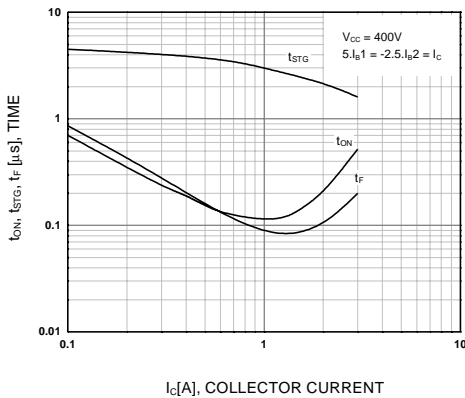
Figure 5. Switching Time
