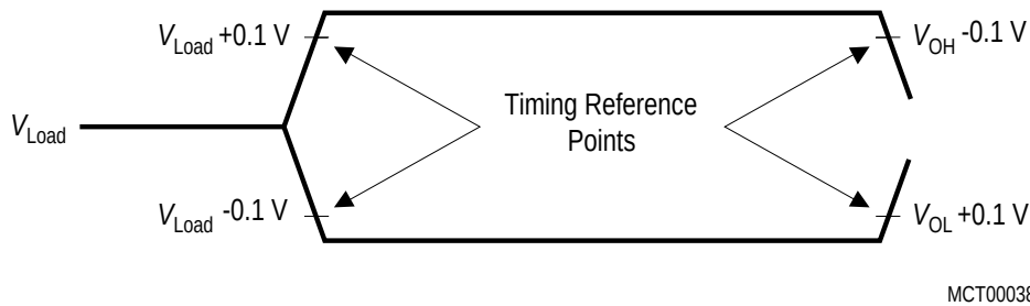
Figure 42 AC Testing: Input, Output Waveforms
