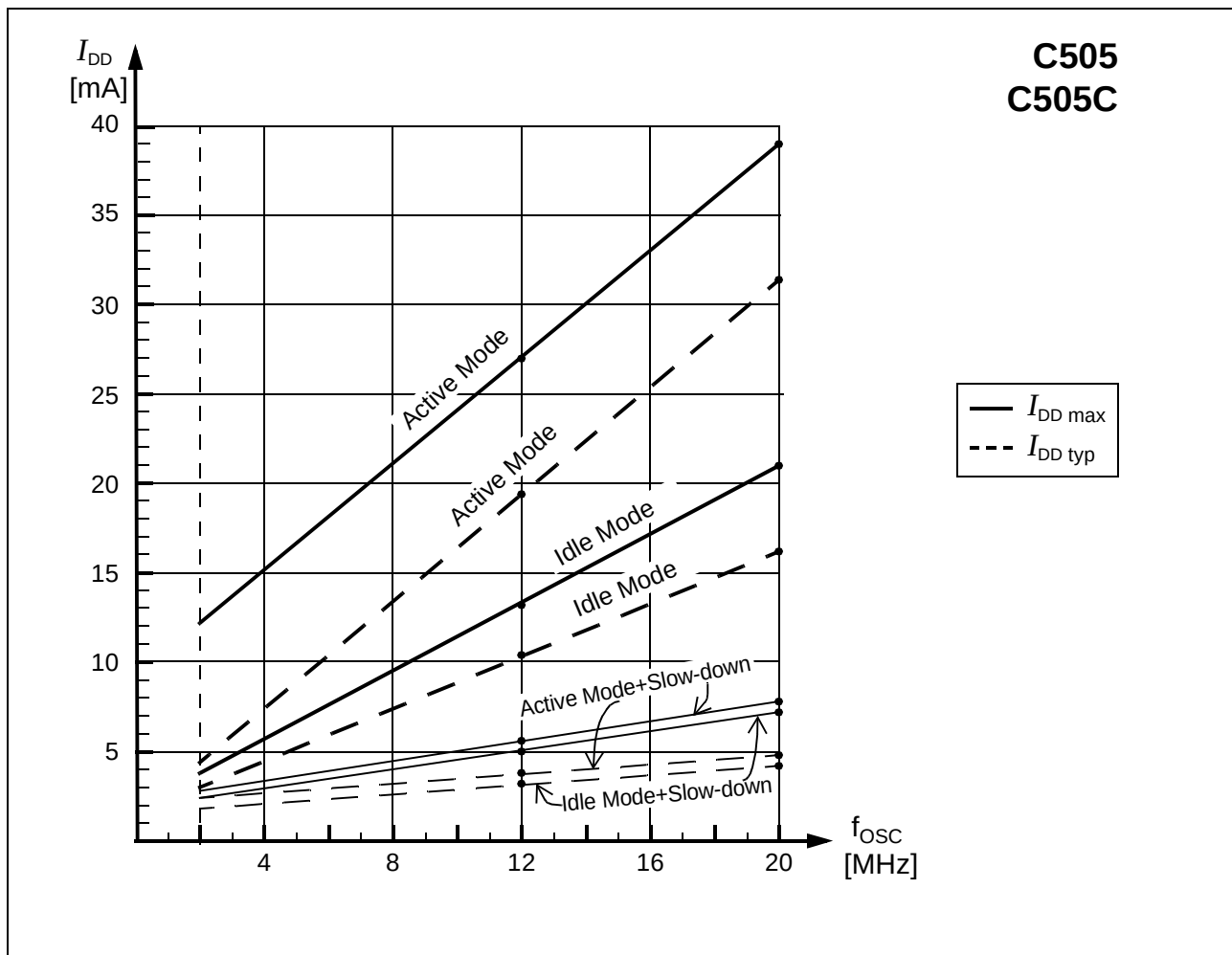
Figure 29 I_{DD} Diagram of C505 and C505C
