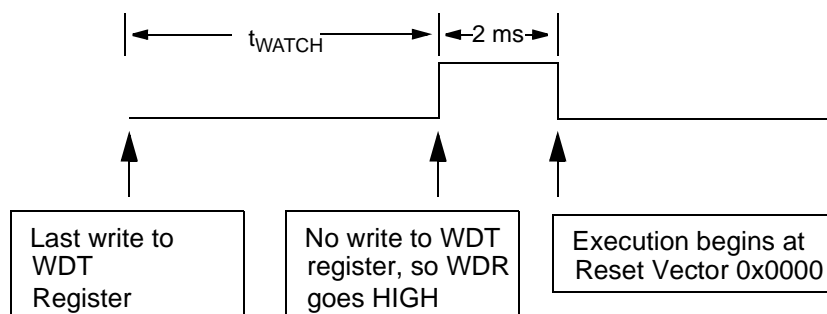
Figure 7-1. Watchdog Reset
