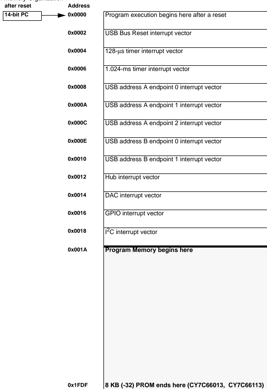
Figure 5-1. Program Memory Space with Interrupt Vector Table
