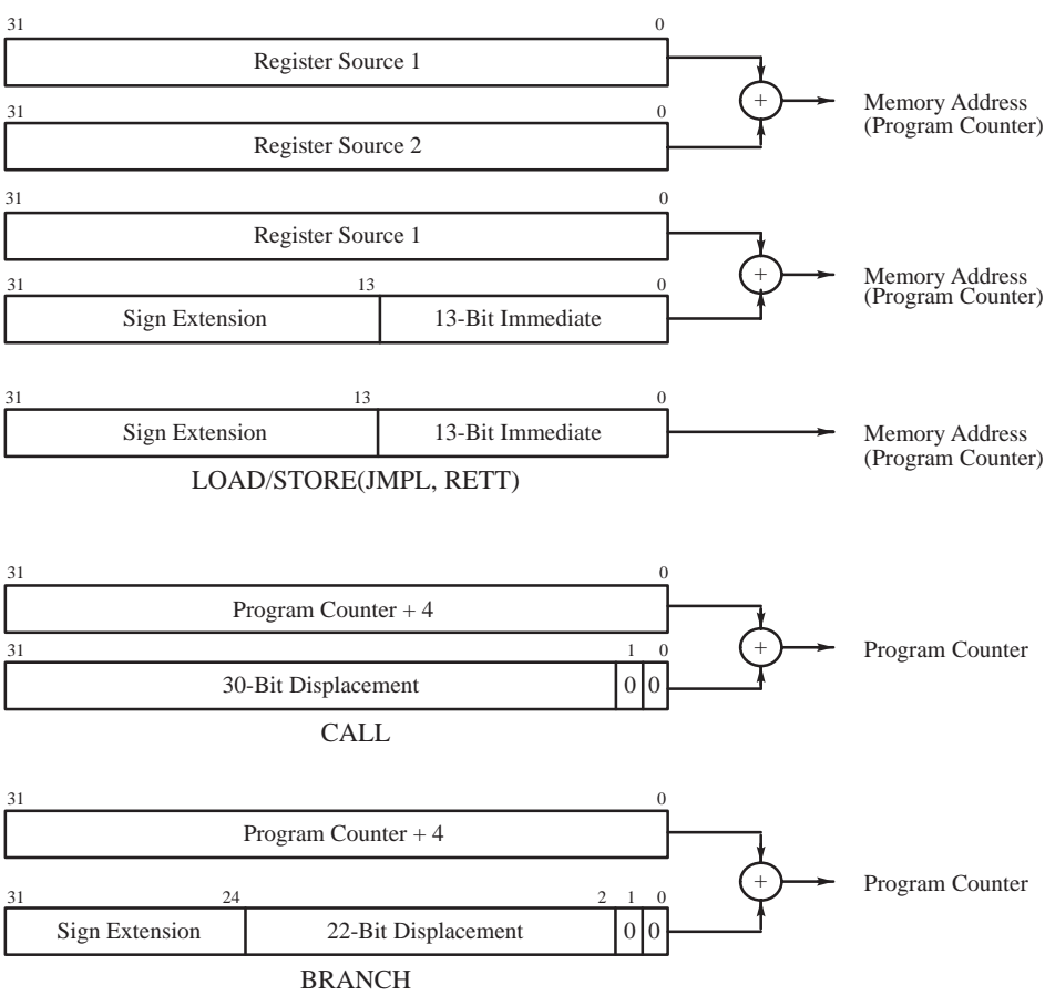
Figure 17. Address Generation
