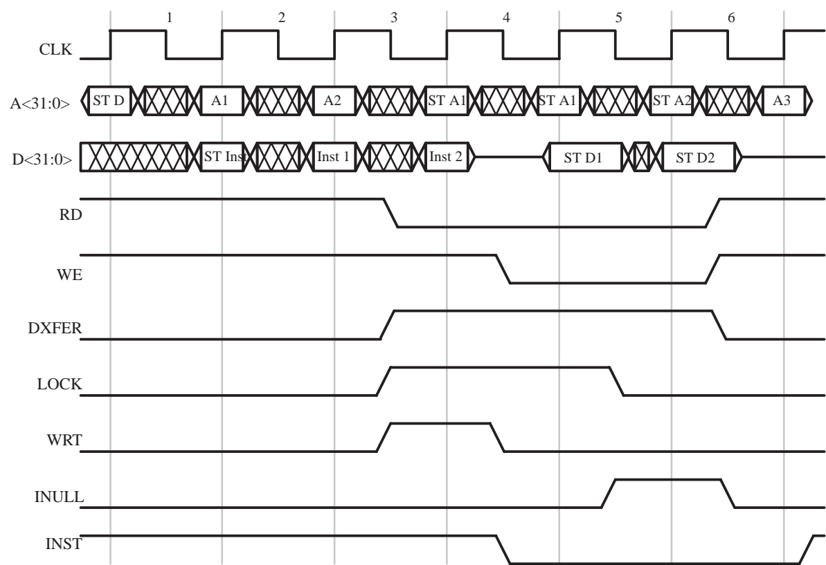
Figure 39. Store Double Integer Timing
