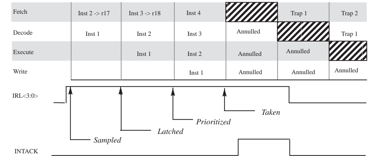
Figure 61. Best-Case Interrupt Response Timing (one cycle instruction)
