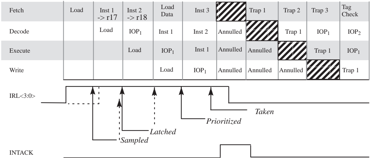
Figure 62. Double Cycles Instruction Interrupt Response Timing (ex: Load)
