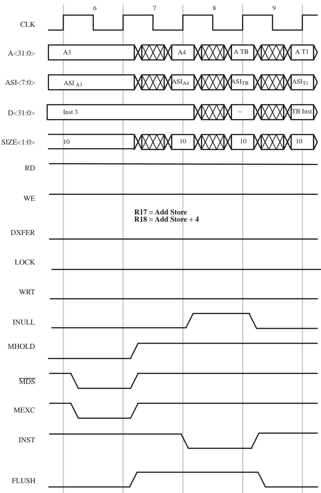
Figure 56. Store double with Memory Exception on 2nd data address (page 2 of 2)
