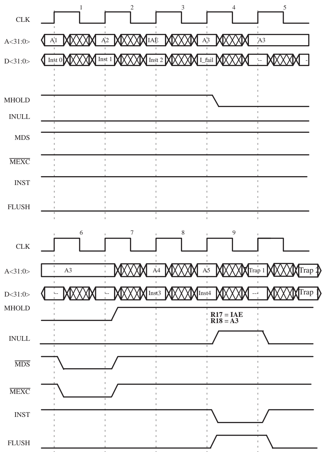
Figure 49. Instruction Memory Access Exception Timing
