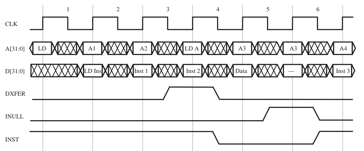
Figure 36. Load Single with Interlock Timing
