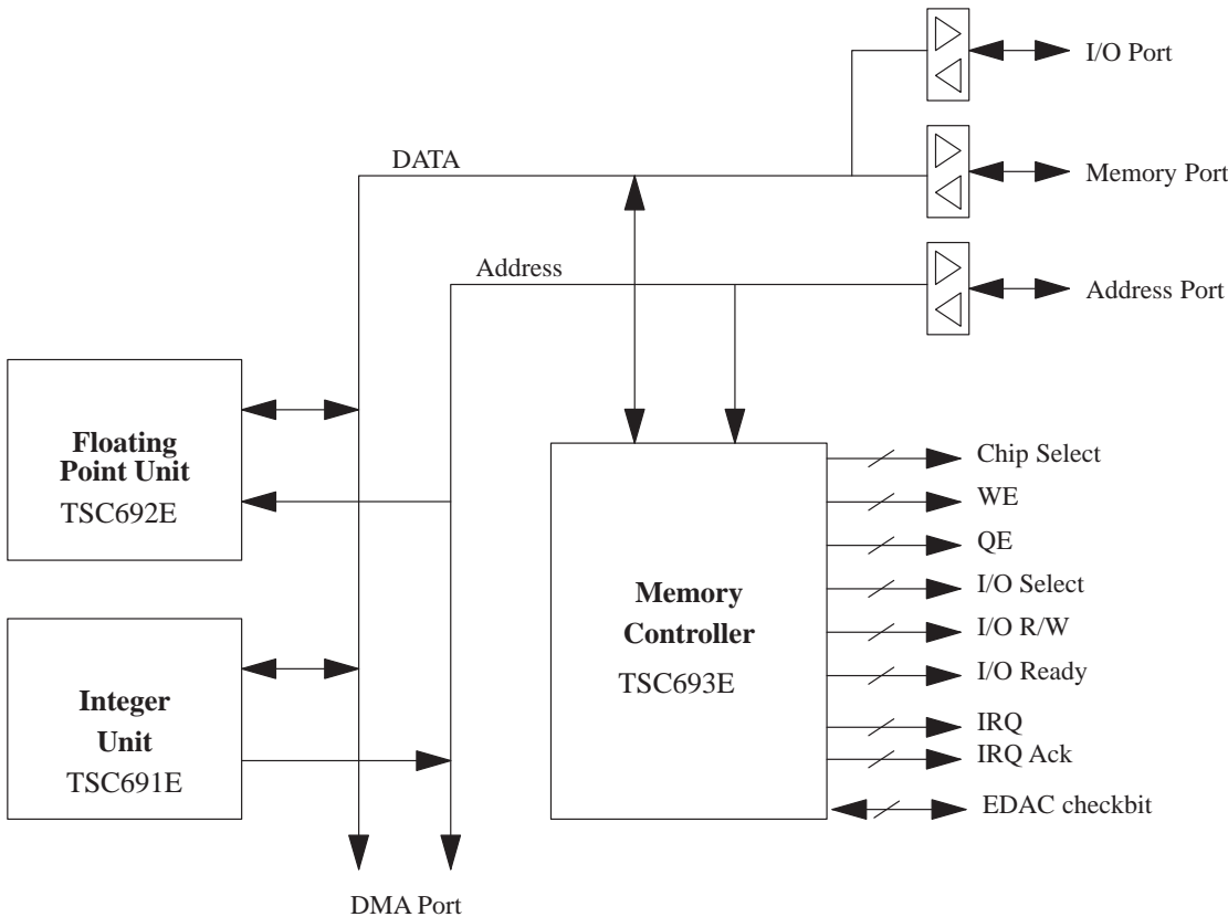
Figure 1. ERC32 Architecture
