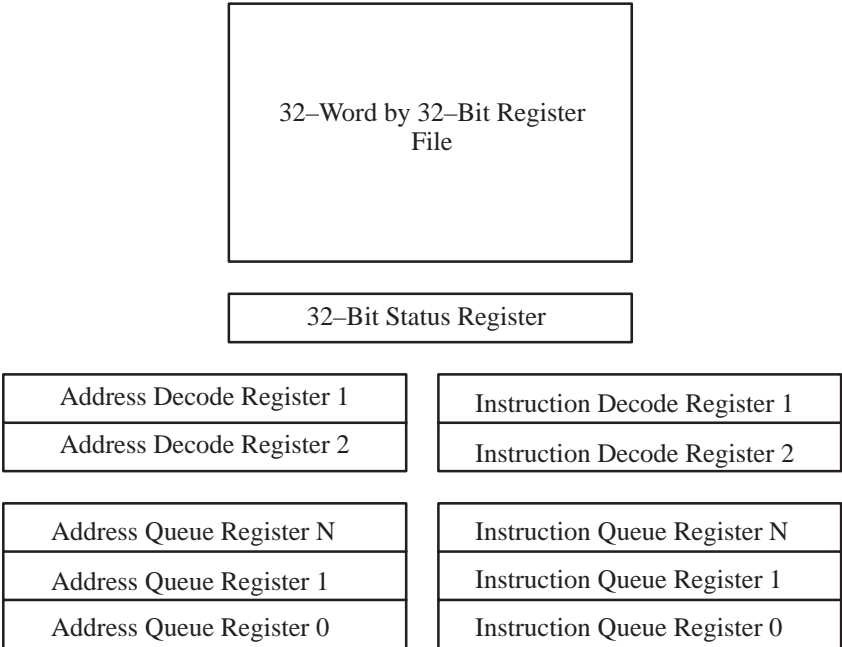
Figure 66. Coprocessor Register Model
