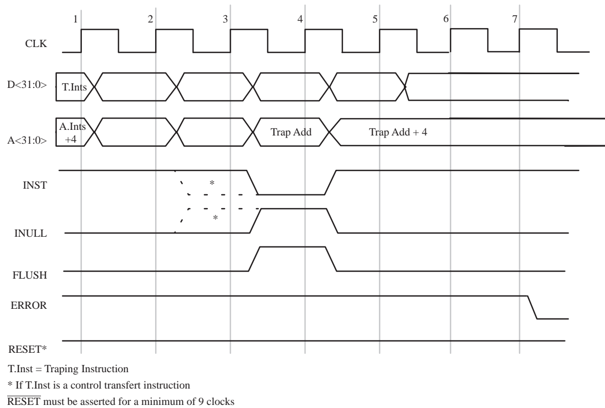
Figure 60. Error/Reset Timing
