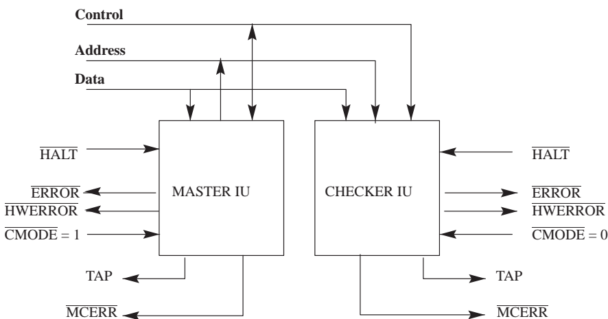
Figure 67. Master/Checker configuration
