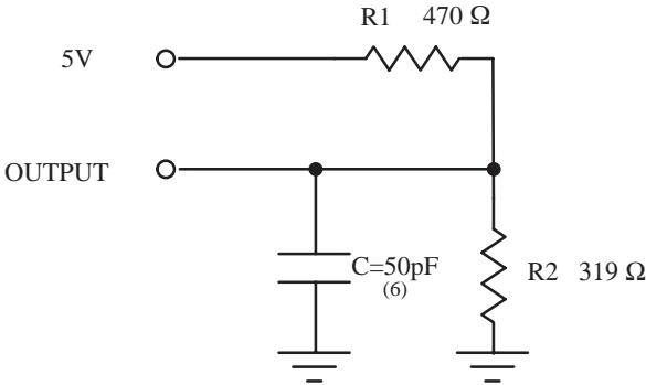
TEST LOAD
