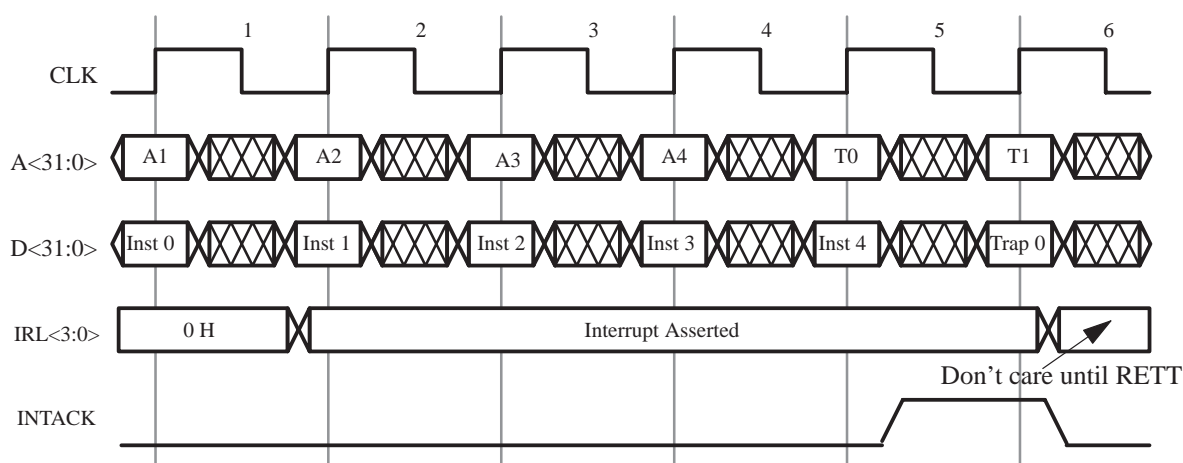
Figure 58. Asynchronous Interrupt Timing
