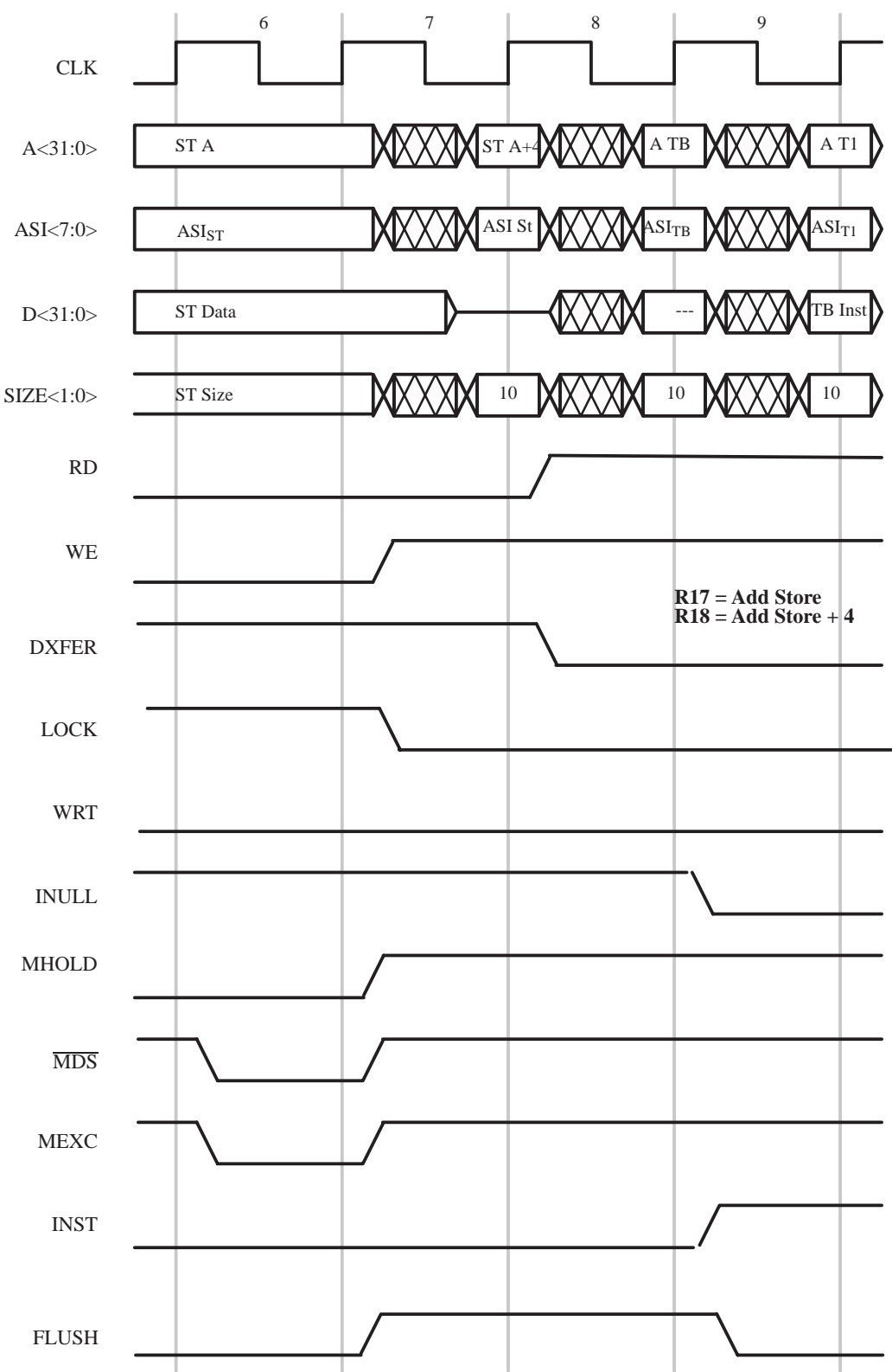
Figure 54. Store double with Memory Exception on 1st data address (page 2 of 2)
