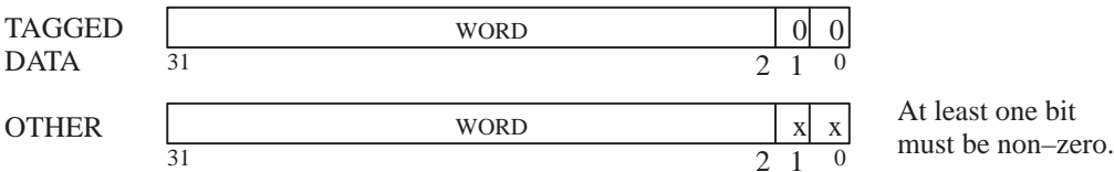
Figure 18. Tagged Data Example
