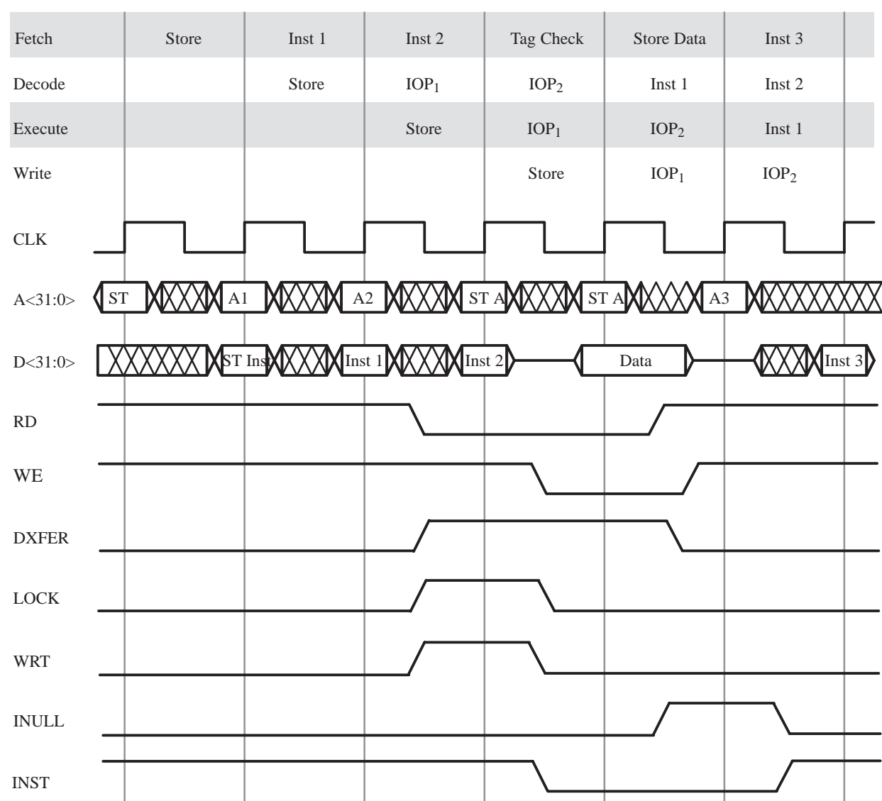
Figure 27. Pipeline with One Triple-Cycle Instruction (Store)
