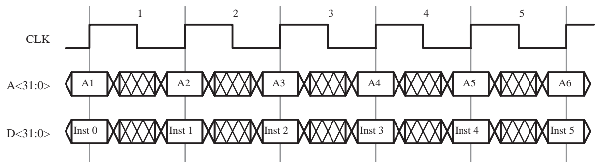
Figure 34. Instruction Fetch
