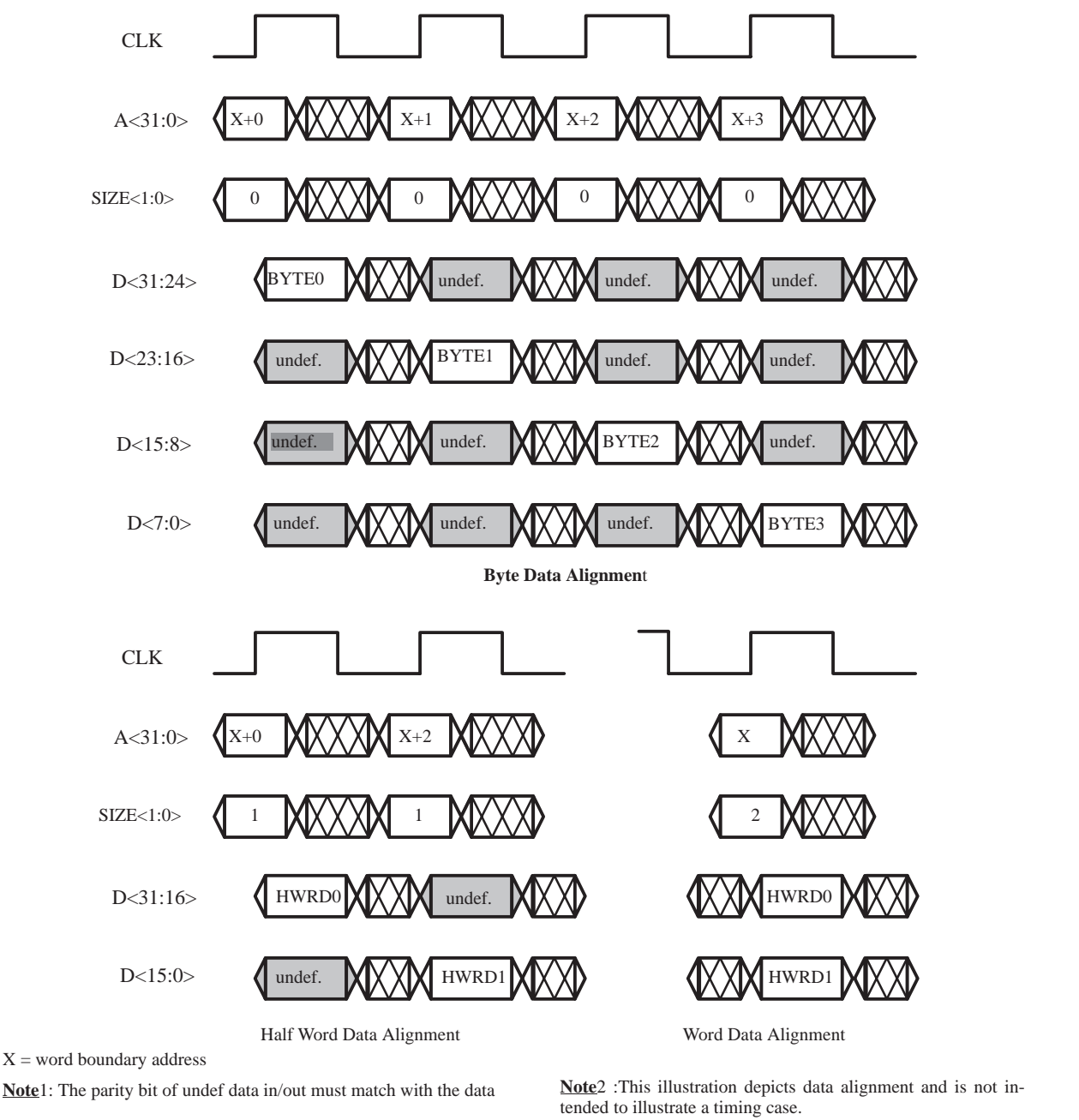
Figure 33. Data Bus Contents During Data Transfers
