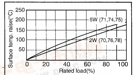
Applied power vs. surface temp.(Example)
